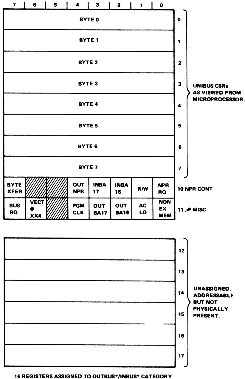
Figure 3-2 Microprocessor Registers
