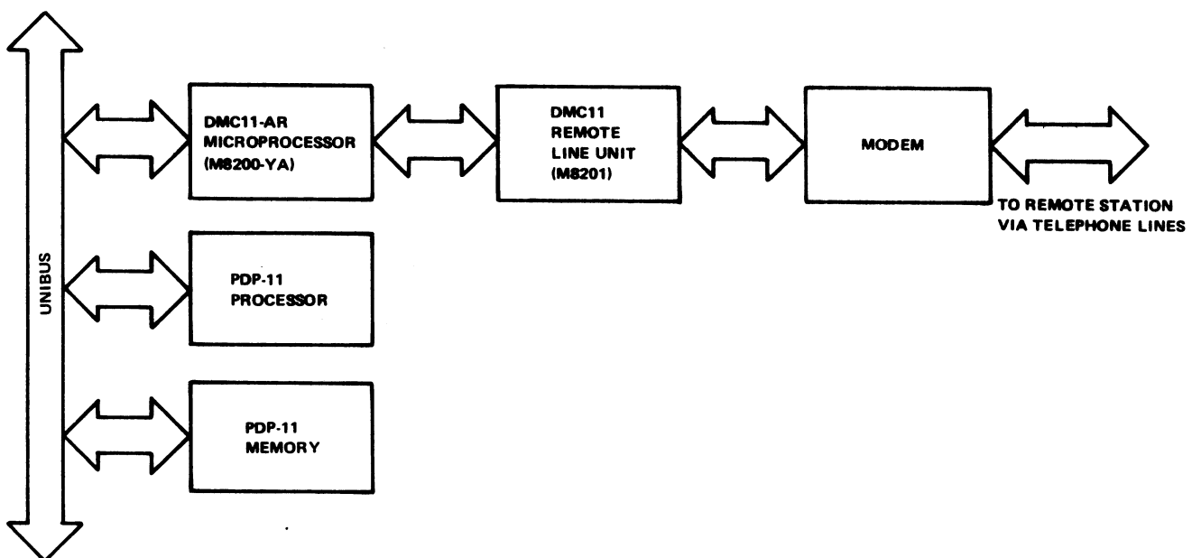
Figure 1-1 DMC11 Remote Line Unit Interface
