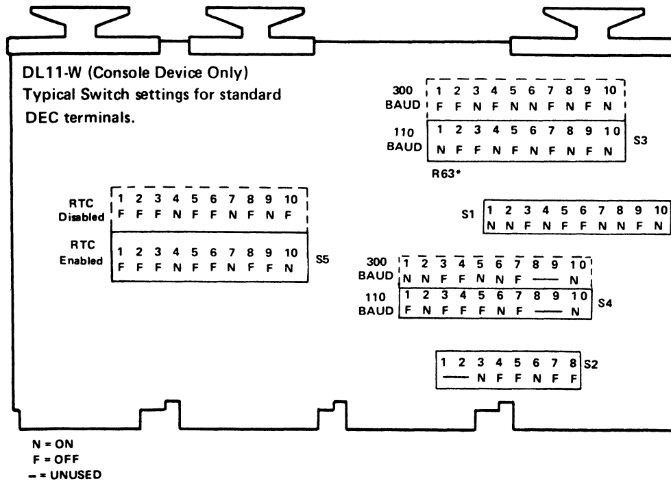
Figure 2-3 Typical Switch Settings
