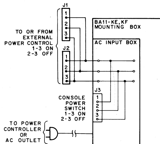
Figure 3-3 Power Control
