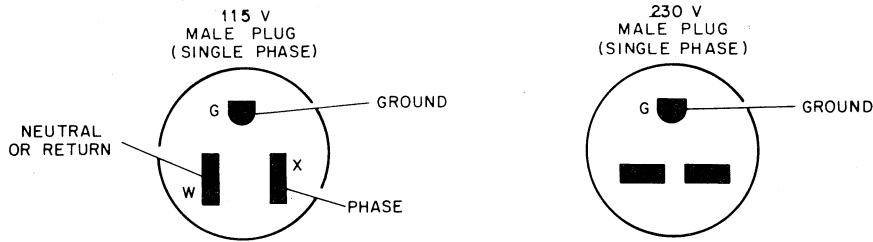
CONNECTOR SPECIFICATIONS
