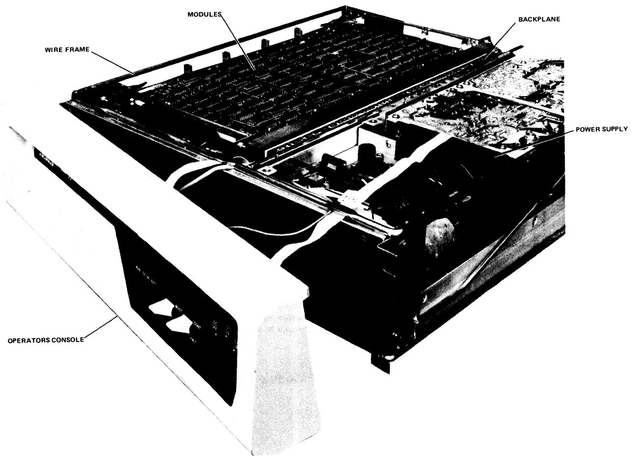
Figure 5-6 Computer Subassemblies of BA11-L Mounting Box
