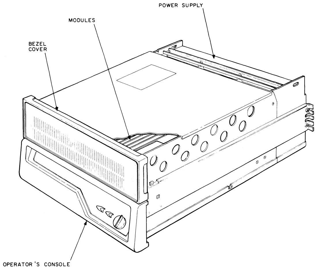
Figure 5-7 Computer Subassemblies of BA11-K Mounting Box
