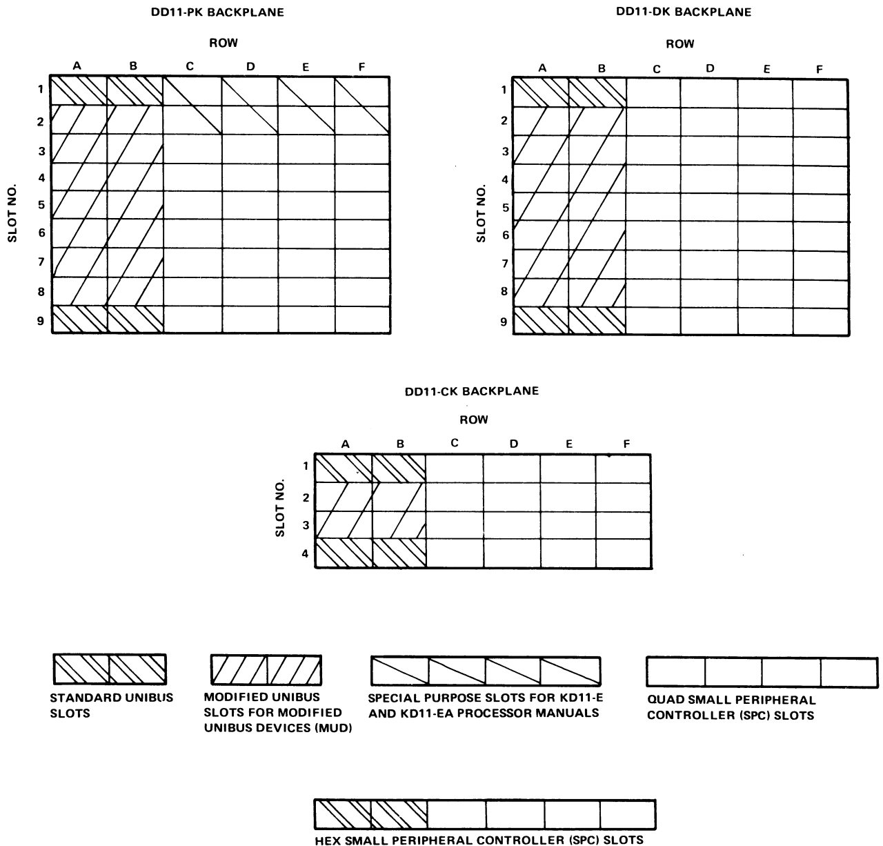
Figure 4-1 PDP-11/34 Backplanes
