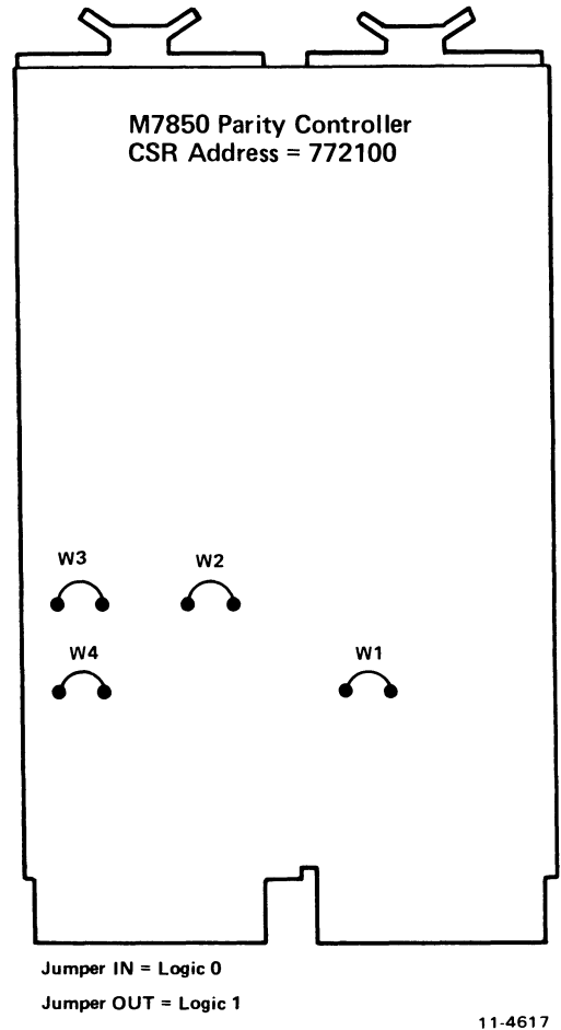
Figure 5-9 Typical Jumper Placement and Switch Settings of Modules (Sheet 1 of 9)
