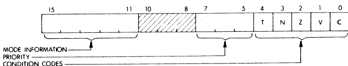
Figure 2-4 Processor Status Word
