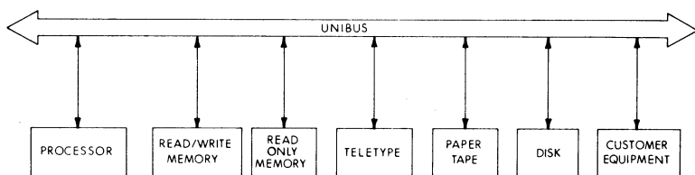
Figure 5.1 PDP-11 System Simplified Block Diagram
