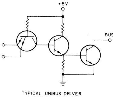
Figure 6-4 Typical Transmitter Circuit
