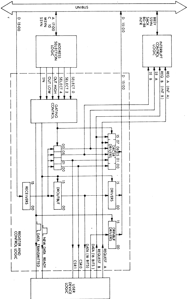
DR11-C Interface, Block Diagram
