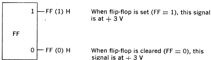
Figure 6-2 Flip-flop signals
