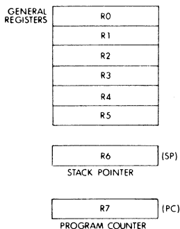
Figure 2-3 General Registers
