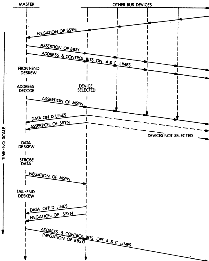
Figure 5-8 Typical DATI or DATIP Cycle
