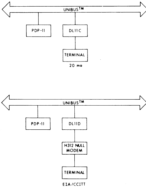
Interfacing a Local Terminal
