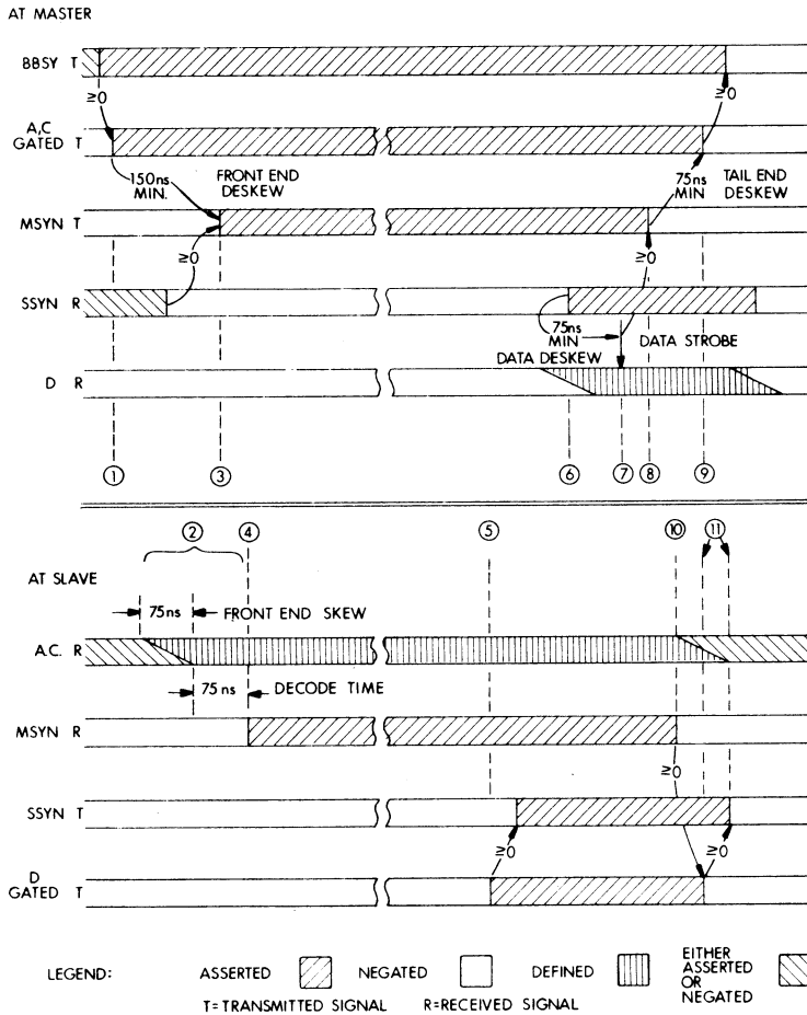
Figure 5-9 Typical DATI Transaction
