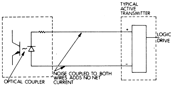
TTY RECEIVER WIRED AS PASSIVE
