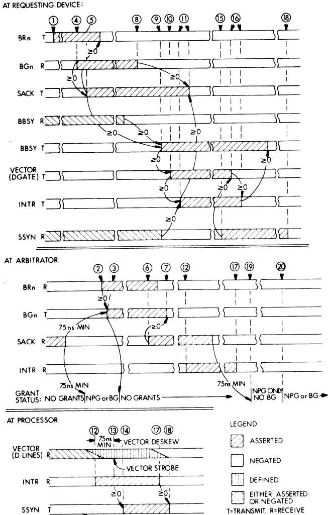
Figure 5-15 Typical Interrupt Transaction
