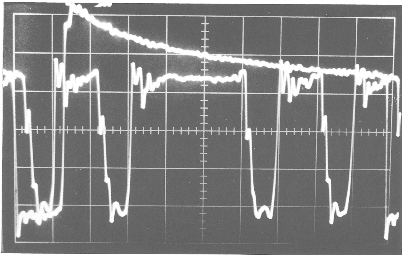
Figure 19 Current Delay 100 ns/cm @ 1 V/cm
