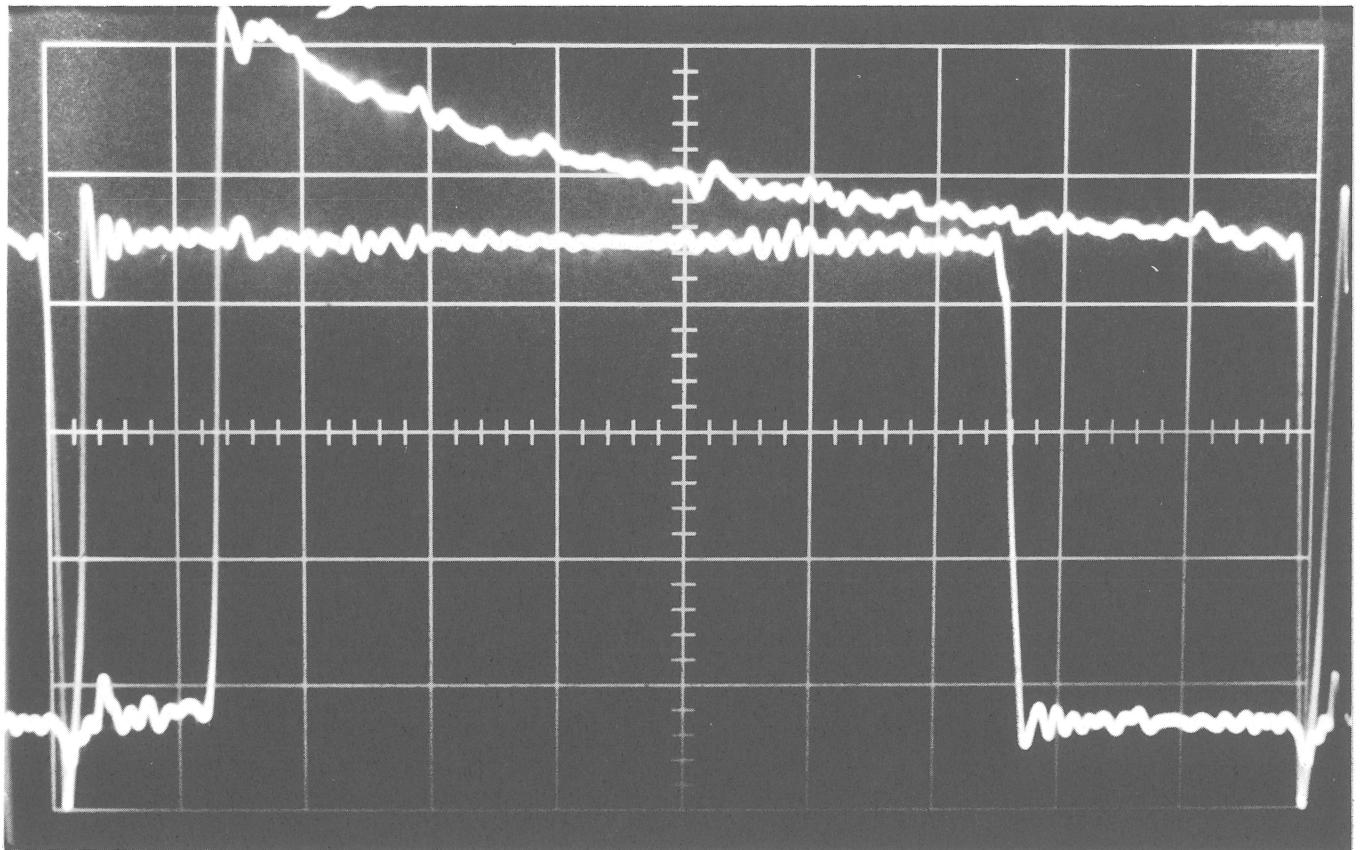
Figure 6 Write Time 100 ns/cm @ 1 V/cm
