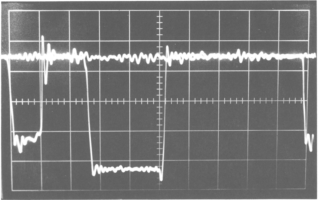
Figure 5 Pause Time 100 ns/cm @ 1 V/cm
