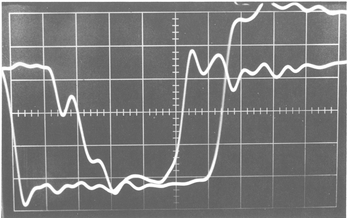
Figure 13 Current Start 20 ns/cm (0.2 \mu s X10) @ 1 V/cm
