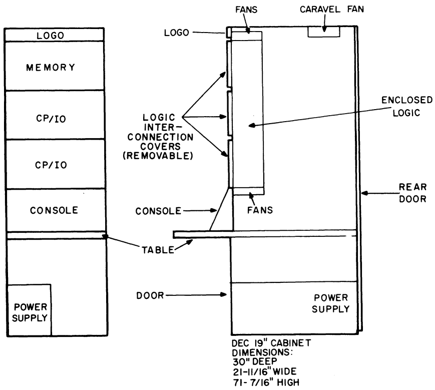
Figure 2-1 PDP-15/10 System Configuration Diagram
