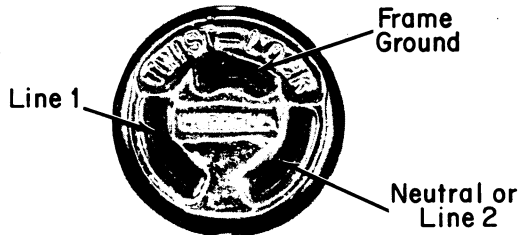
Figure 3-5 Hubbell Wall Receptacle Connector Diagram
