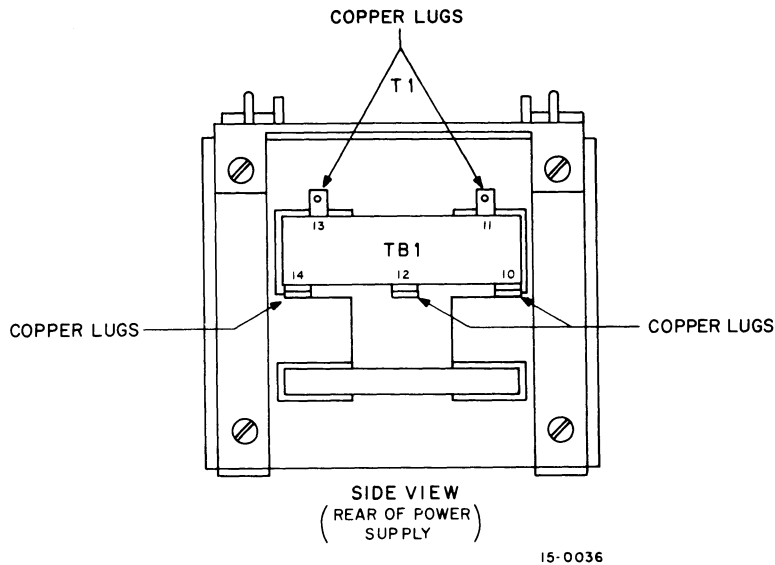
Figure 4-7 Transformer Terminal Connector Diagram (Side View)
