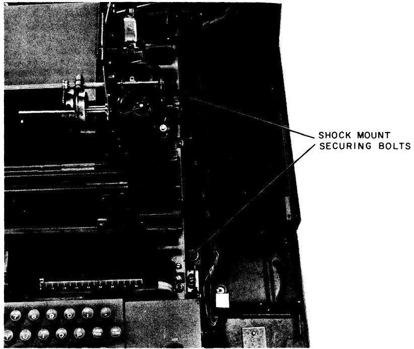
Figure 4-3 35 ASR and 35 KSR Right-Side Shock Mount Bolts
