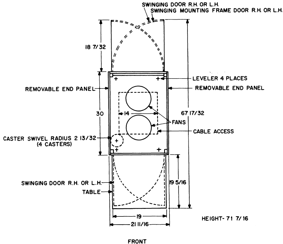
Figure 3-1 Basic PDP-15 Cabinet
