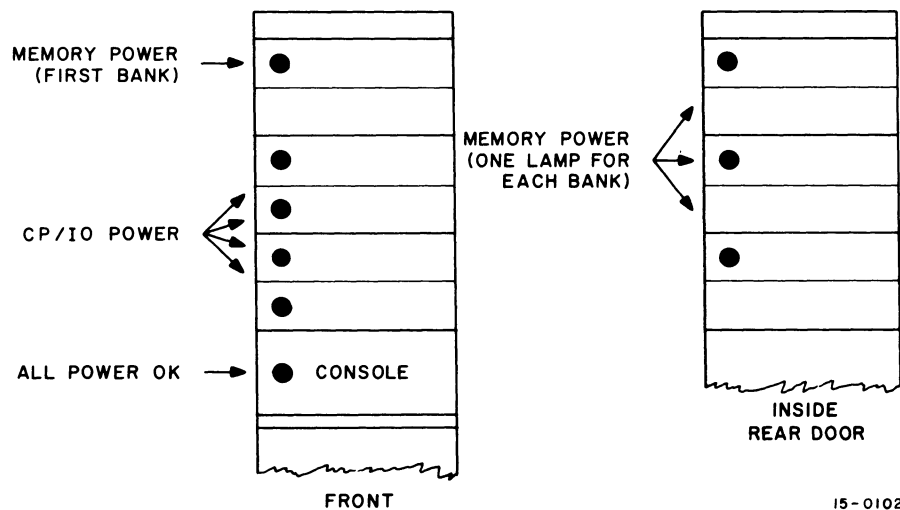
Figure 4-8 DC Power Lamp Locations
