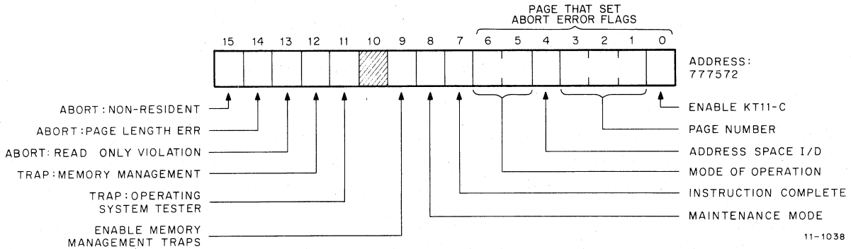
Figure 2-10 Format of Status Register 0 (SR0)
