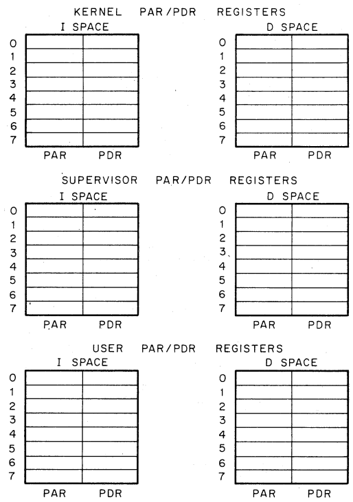
Figure 2-5 KT11-C Memory Management Unit PAR/PDR Registers
