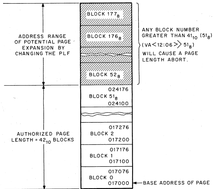
Figure 2-8 Example of an Upward Expandable Page
