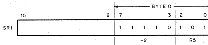
a. AUTO-DECREMENT R5 BY 2, SOURCE CALCULATION
