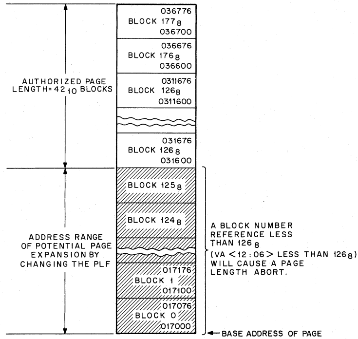
Figure 2-9 Example of a Downward Expandable Page
