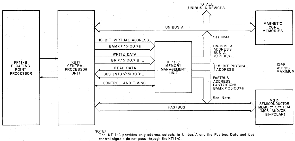
Figure 3-1 KT11-C System Hardware Interface
