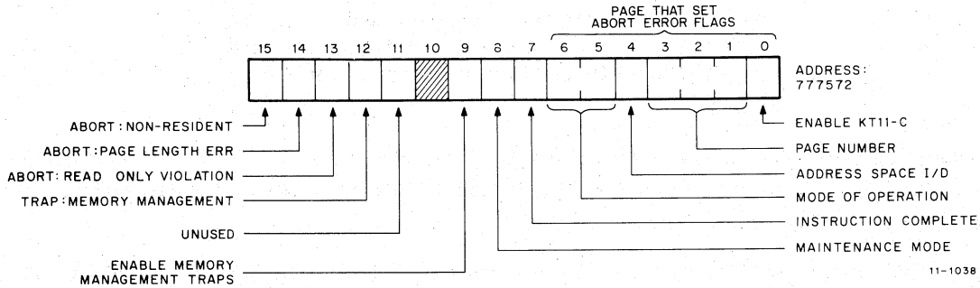
Figure 2-10 Format of Status Register 0 (SR0)
