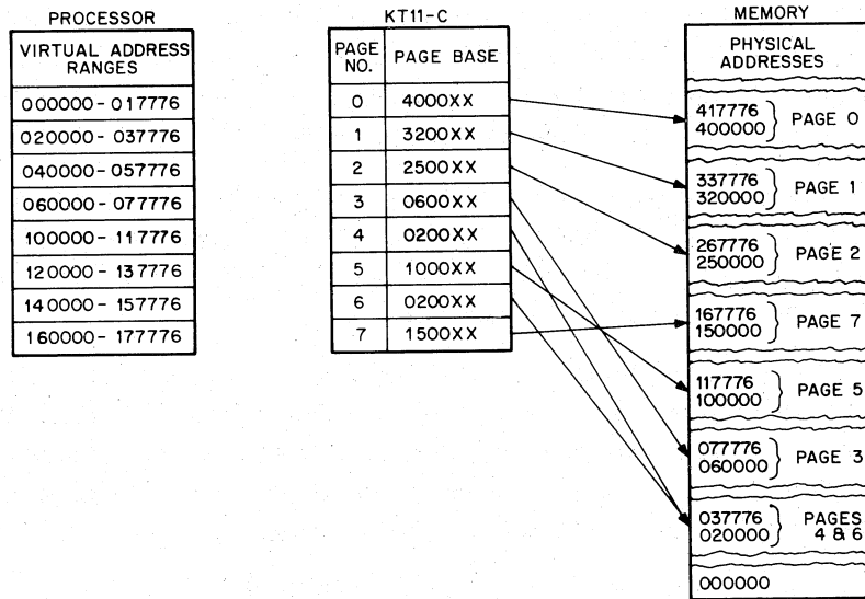
Figure 2-2 Relocation of a 32K-Word Program into 124K-Word Physical Memory
