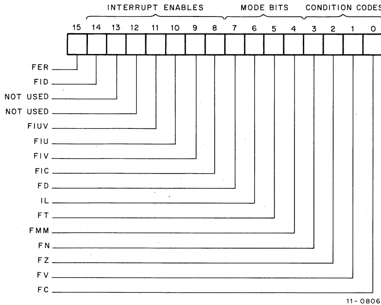
Figure 3-3 Status Register Format
