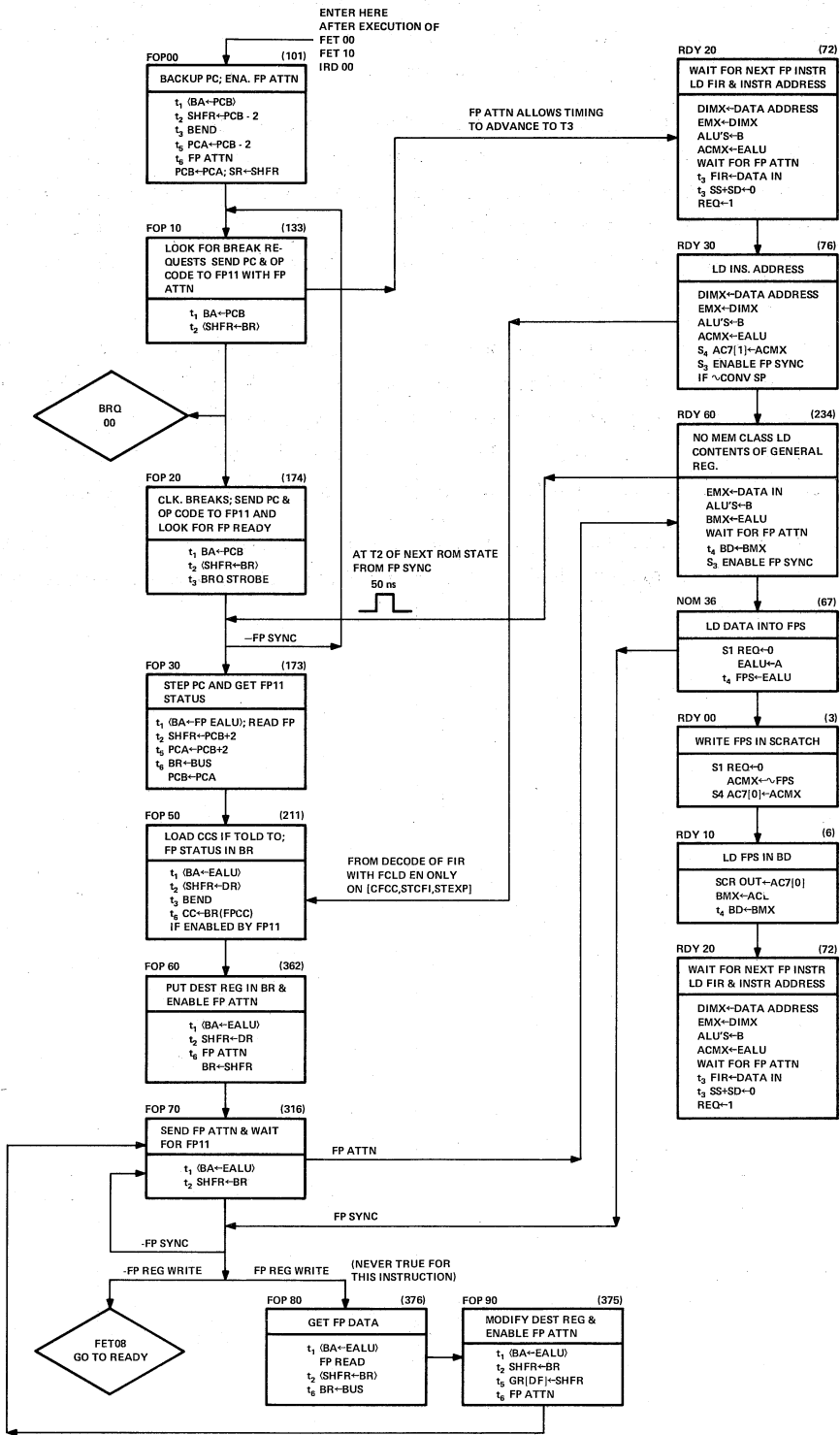
Figure 2-4 LD FPS Instruction Interaction – Mode 0
