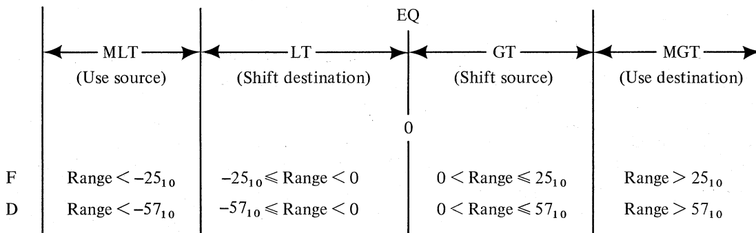
Figure 5-1 Exponent Magnitudes
