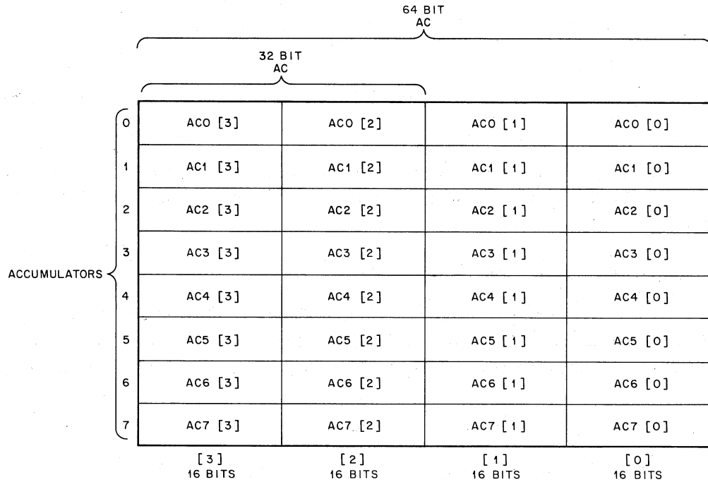
Figure 1-3 Accumulator Configuration
