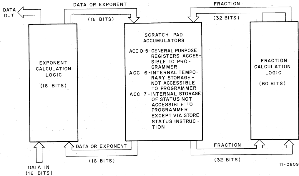
Figure 1-2 FP11 Simplified Block Diagram
