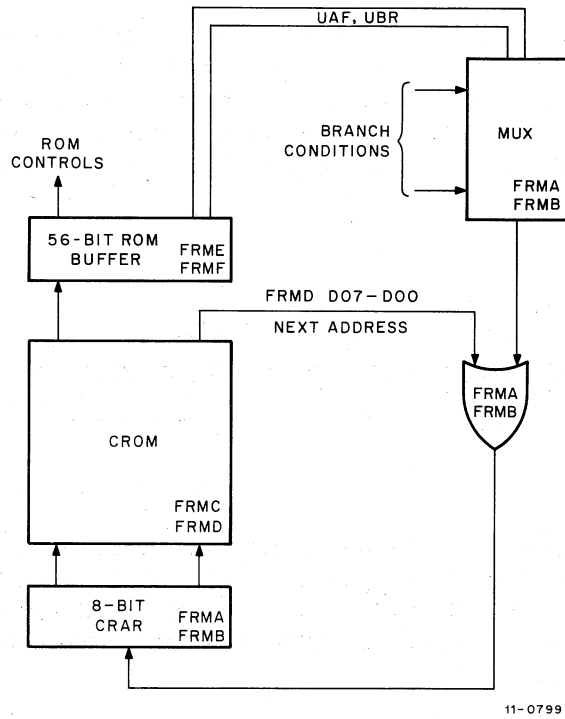
Figure 4-2 Control ROM Simplified Block Diagram
