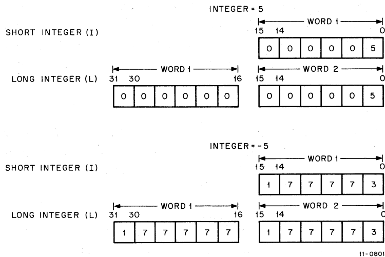
Figure 3-1 Integer Formats
