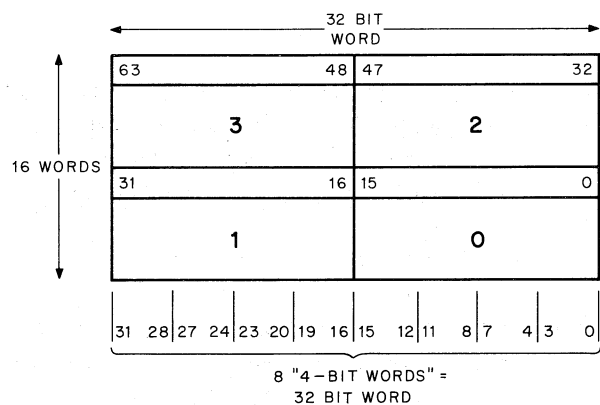
Figure 6-2 Scratchpad Configuration
