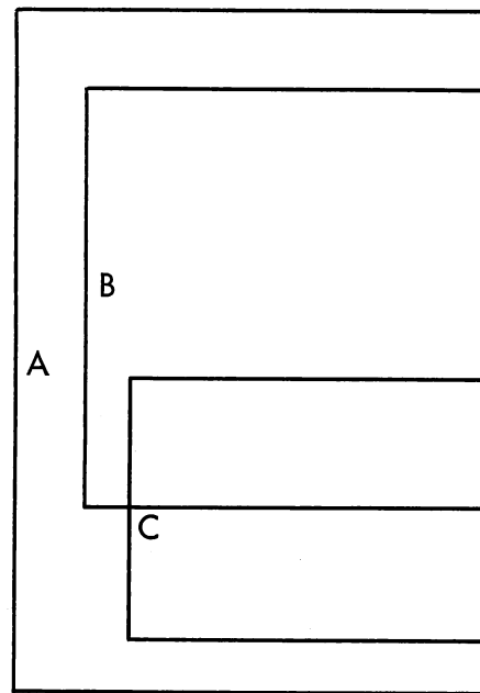
Invalid DO Loop Nest
