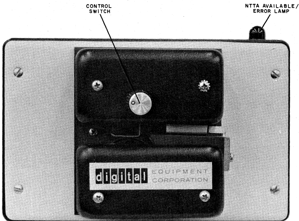
Figure 3-2 PR68B Reader
