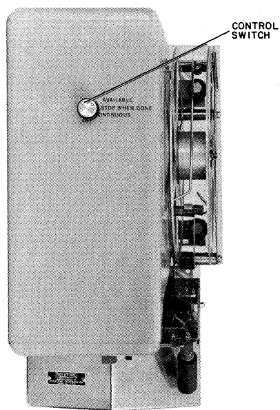
Figure 3-5 PP67C/D Punch Controls
