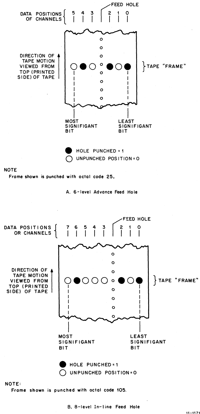
Figure 3-1 Paper-Tape Formats
