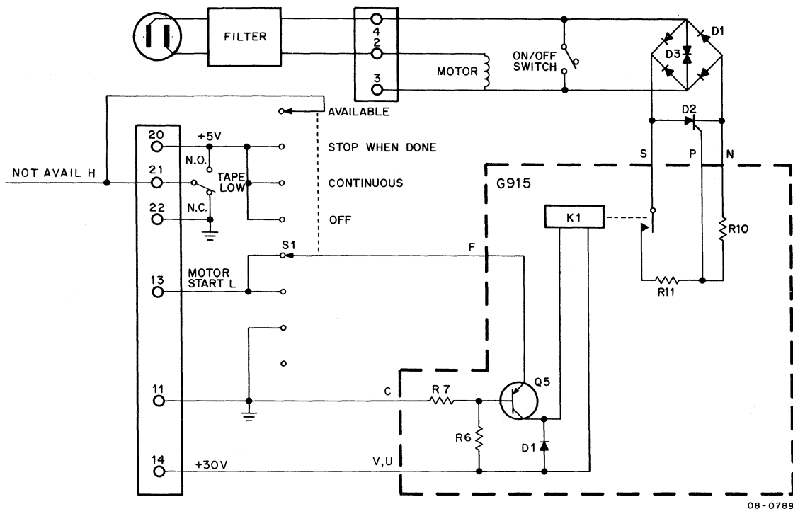
Figure 4-8 Punch Motor Control, Simplified Functional Diagram
