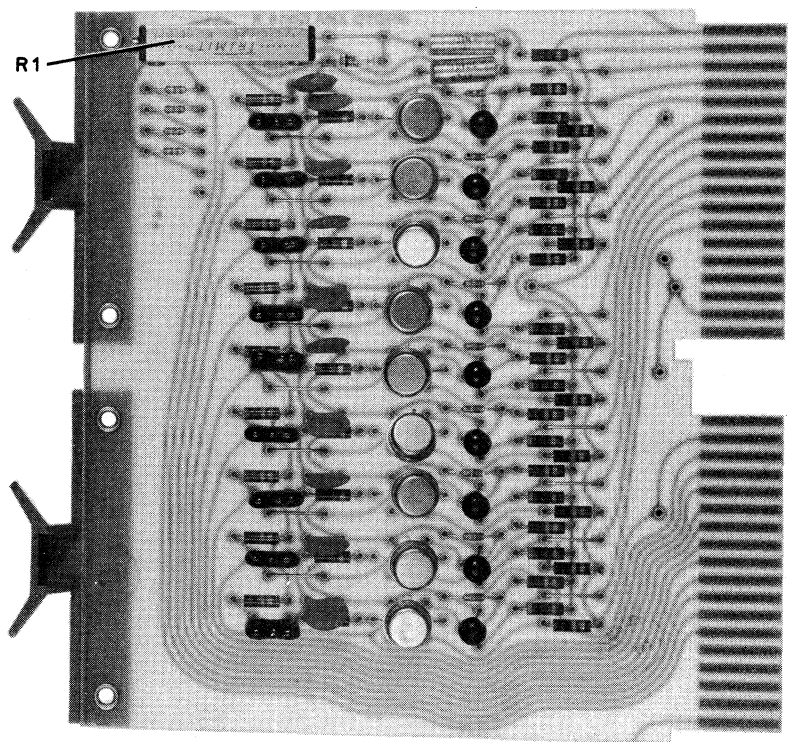
G908 PHOTOAMPLIFIER MODULE
