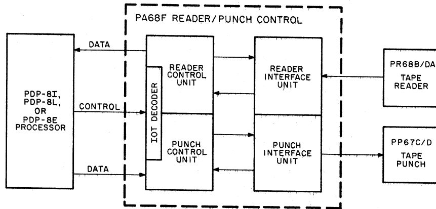
Figure 1-3 Single Reader/Punch System
