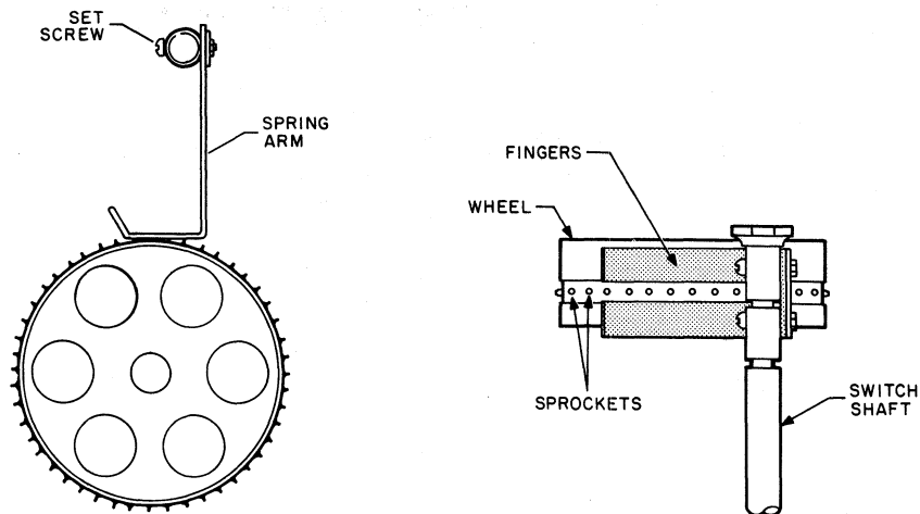
Figure 5-10 Spring Arm Adjustment for PR68B
