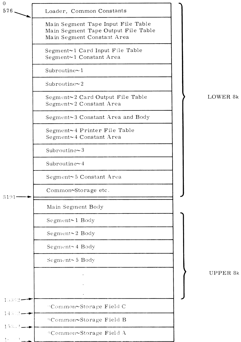
Figure 46. Example of 16k Memory Allocation
