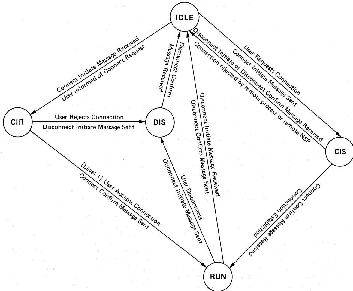
Figure 5-1 Logical Link State Diagram
