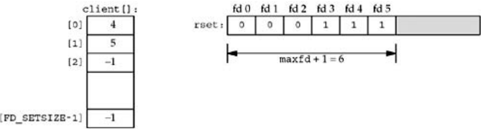
Figure 6.19. Data structures after second client connection is established.
