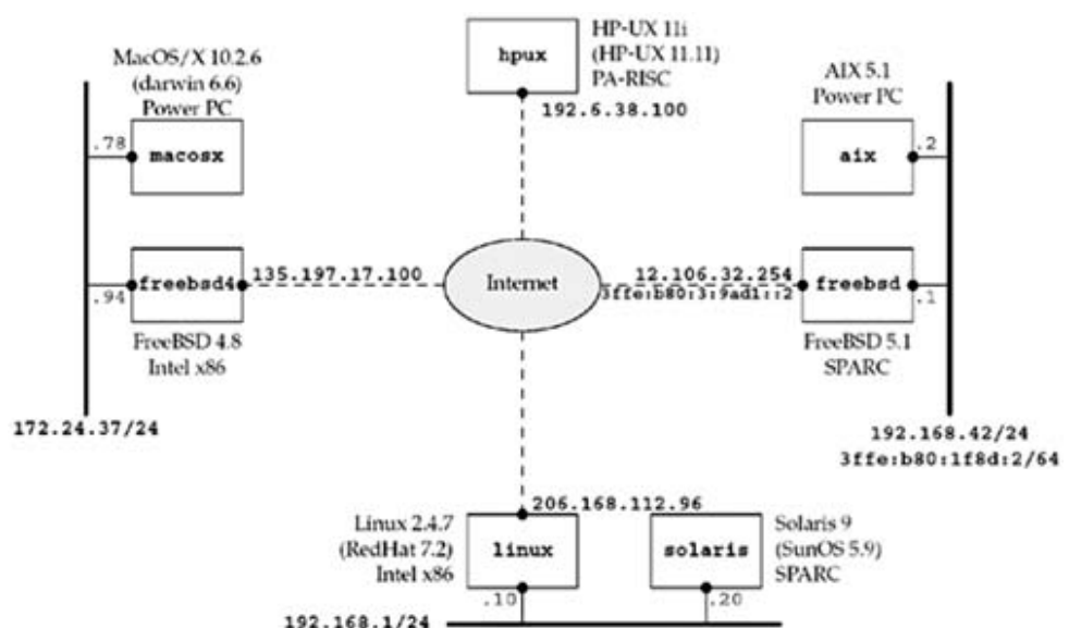
Figure 1.16. Networks and hosts used for most examples in the book
