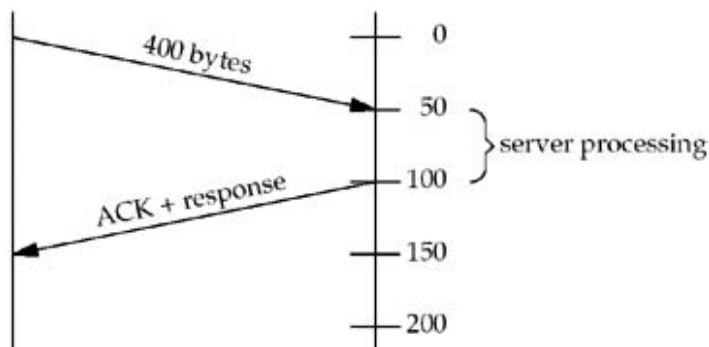
Figure E.8. Using writetv instead of setting the TCP_NODELAY socket option.
