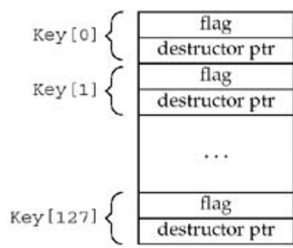
Figure 26.7. Possible implementation of thread-specific data.
