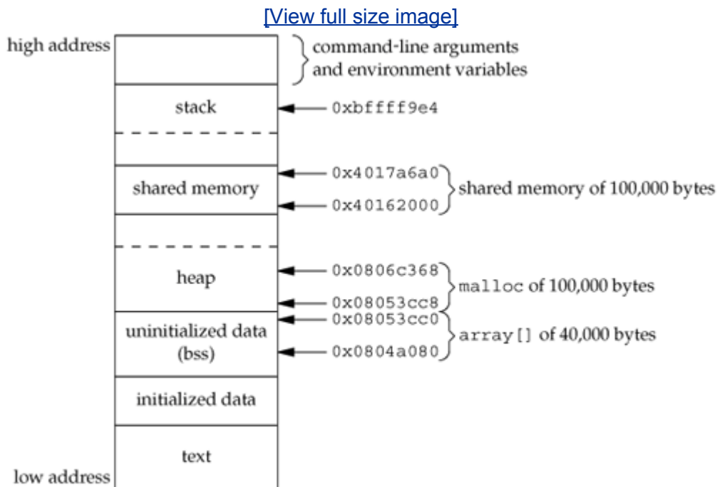
Figure 15.32. Memory layout on an Intel-based Linux system
