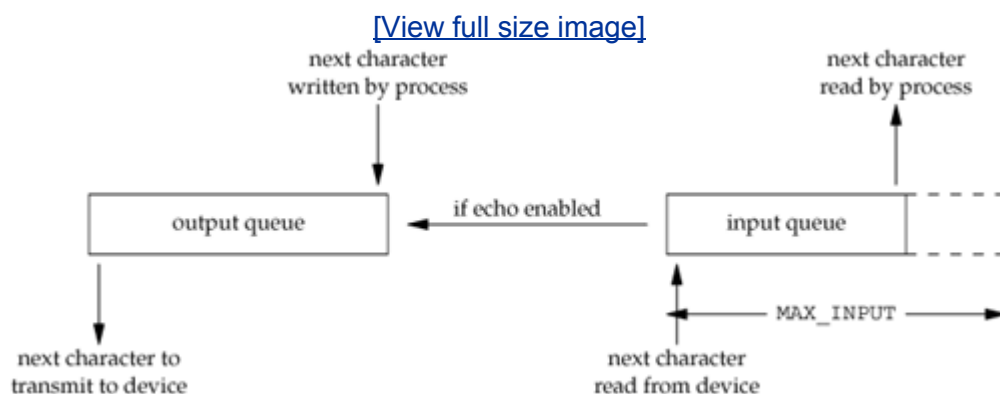
Figure 18.1. Logical picture of input and output queues for a terminal device
