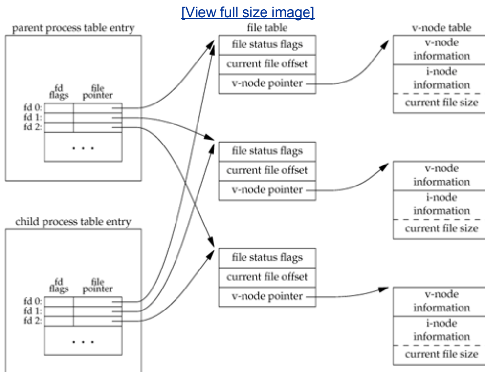
Figure 8.2. Sharing of open files between parent and child after fork
