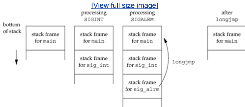
Figure C.10. Stack frames before and after longjmp
