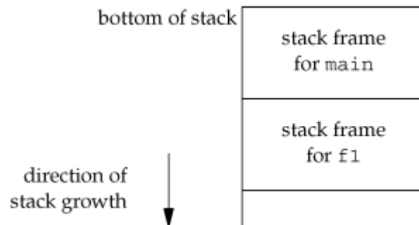
Figure C.8. Stack frames when vfork is called
