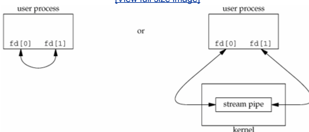
Figure 17.1. Two ways to view a STREAMS pipe
