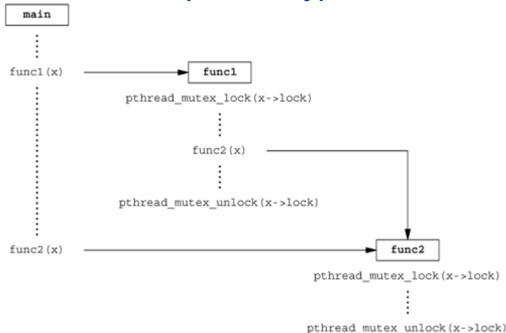
Figure 12.7. Avoiding a recursive locking opportunity
