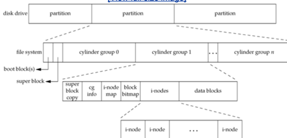
Figure 4.13. Disk drive, partitions, and a file system
