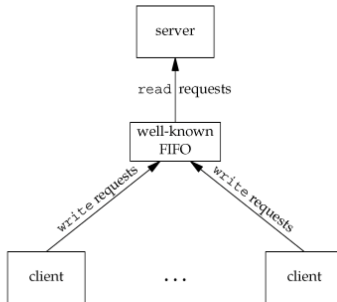
Figure 15.23. Clientserver communication using FIFOs
