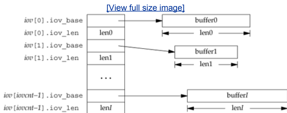
Figure 14.27. The iovec structure for readv and writev
