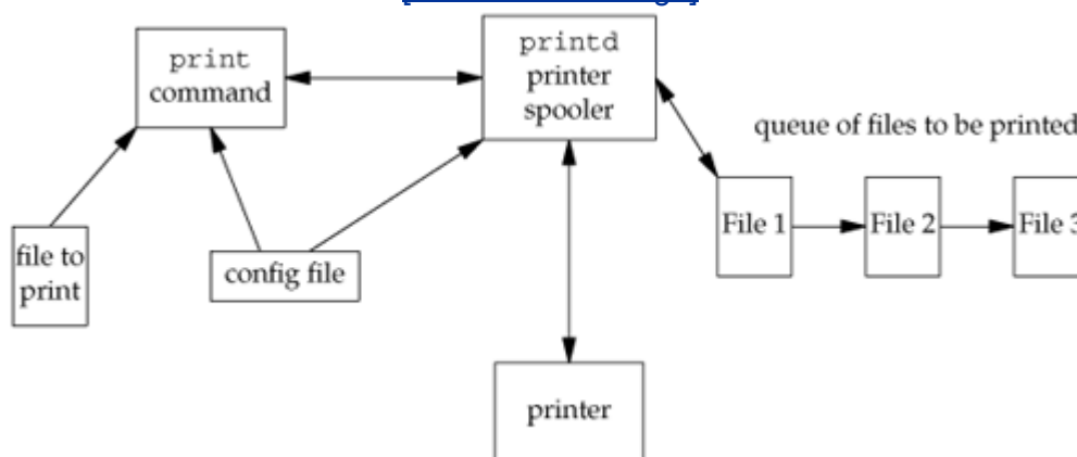
Figure 21.6. Printer spooling components
