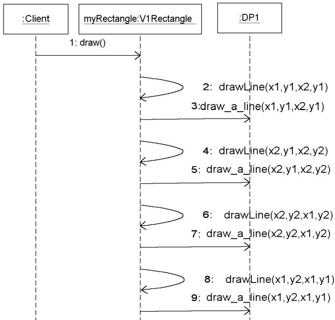
Figure 9-8 Sequence Diagram for new approach.
