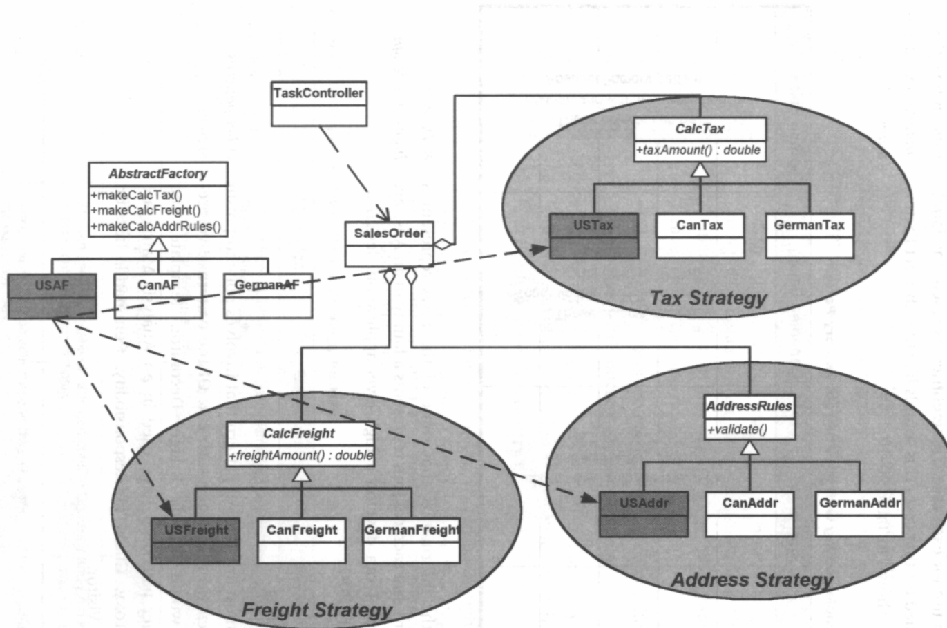
Figure 20-1 Using Strategy patterns with an Abstract Factory.
