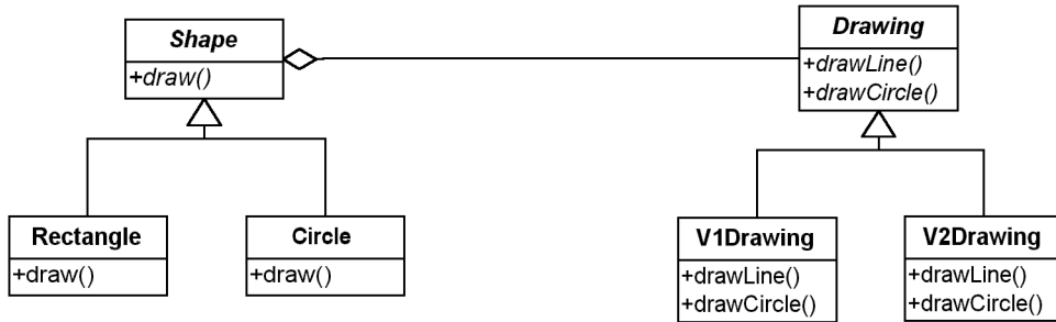
Figure 9-11 Tie the classes together.
