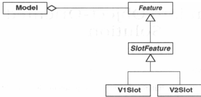
Figure 4-1 The design for slots.
