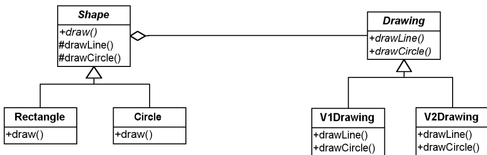
Figure 9-12 Expanding the design.
