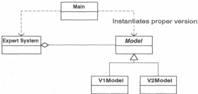
Figure 3-6 Class diagram of my solution! 1
