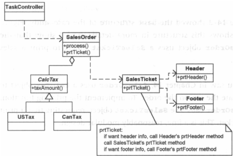
Figure 15-2 SalesOrder using SalesTicket with different options.
