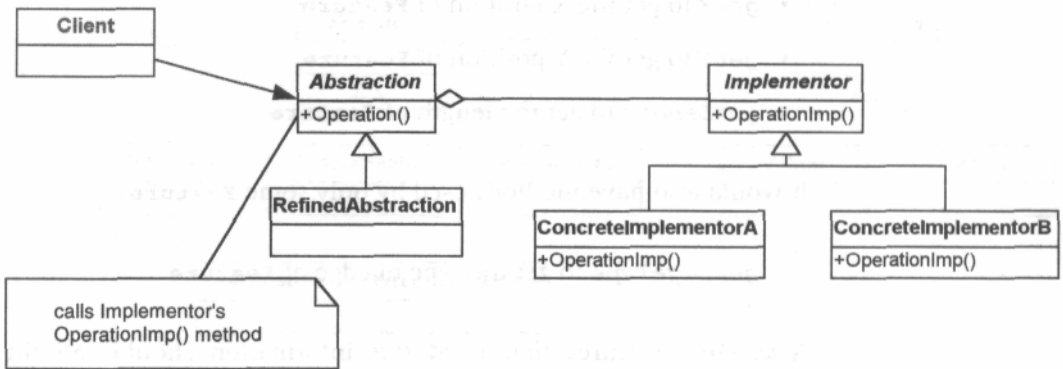
Figure 12-8 The canonical Bridge pattern.
