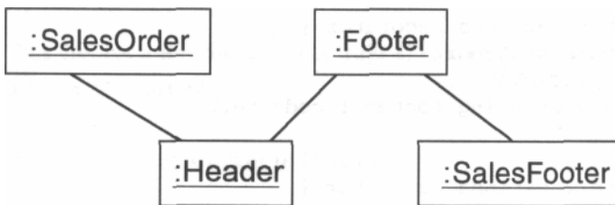
Figure 15-6 An example Decorator object diagram.
