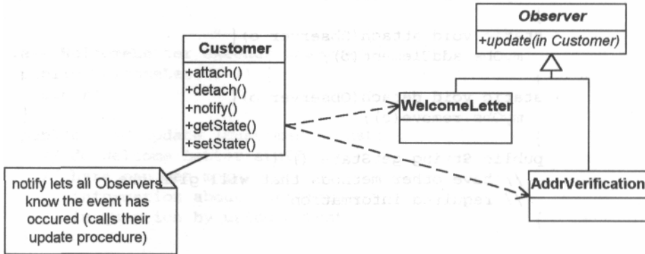
Figure 17-2 implementing Customer with Observer.
