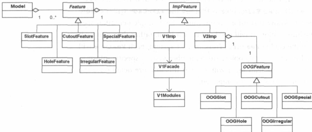
Figure 12-11 After applying the Bridge, Facade, and Adapter.
