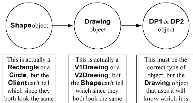
Figure 9-14 There are only three objects at a time.
