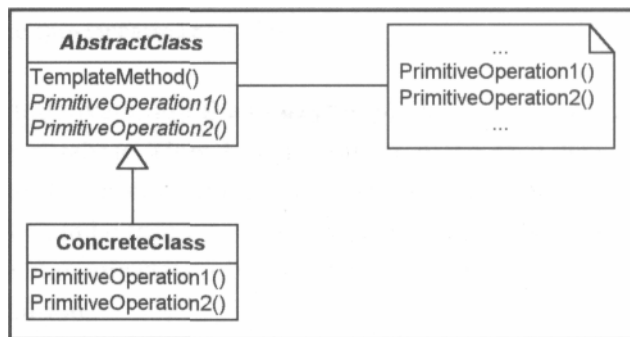
Figure 18-2 Standard, simplified view of the Template Method pattern.
