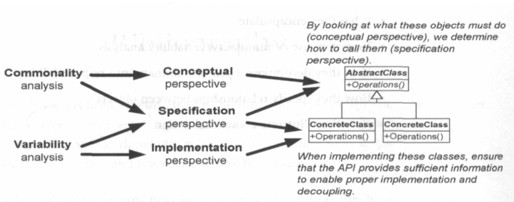
Figure 21-1 The relationships between commonality/variability analysis, perspectives, and abstract classes.
