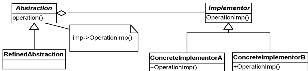
Figure 9-15 Standard, simplified view of the Bridge pattern.
