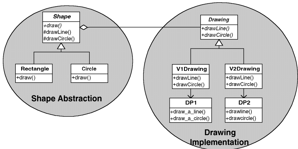
Figure 9-13 Class diagram illustrating separation of abstraction and implementation.
