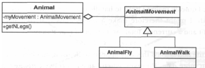
Figure 8-2 Animal containing AnimalMovement object.
