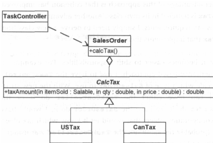
Figure 14-4 Favoring composition over inheritance.
