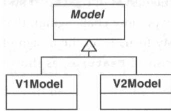
Figure 12-6 Using inheritance to handle the two model types.
