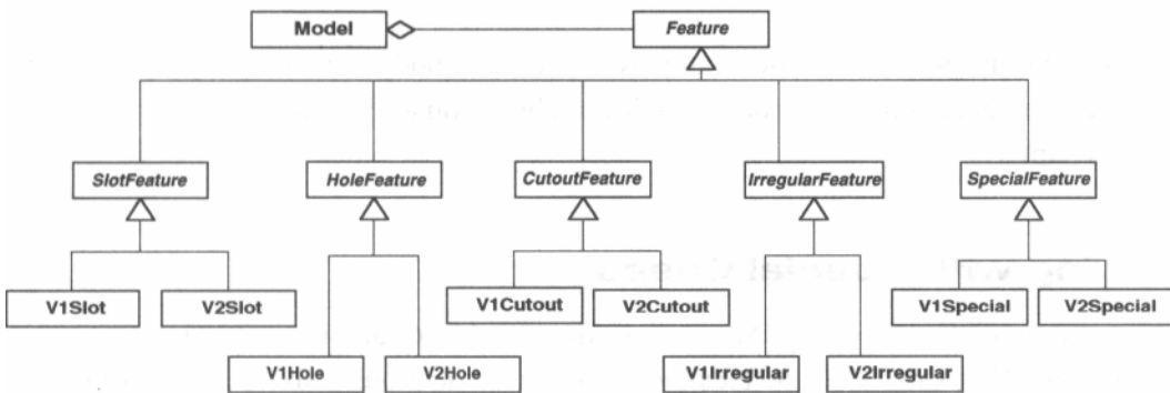
Figure 4-2 Original solution to the problem of extracting information.
