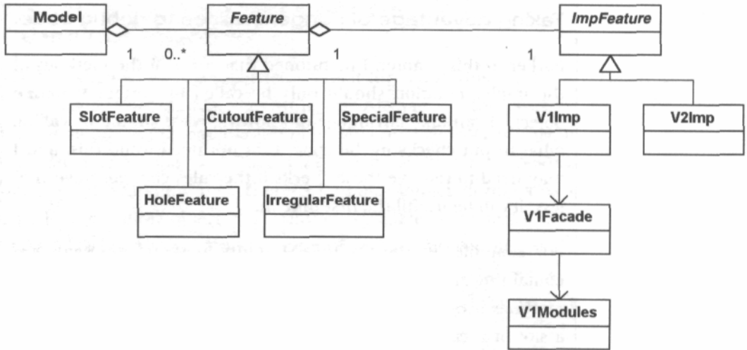
Figure 12-10 After applying the Bridge and Facade patterns.
