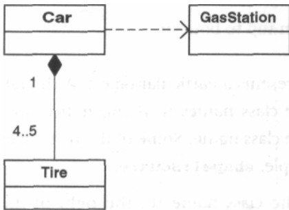
Figure 2-7 The cardinality of the Car-Tire relationship.
