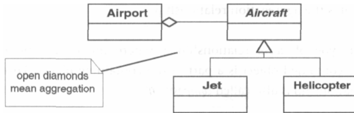
Figure 2-5 The Class Diagram with a Note.
