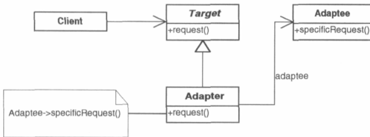
Figure 7-6 Standard, simplified view of the Adapter pattern.
