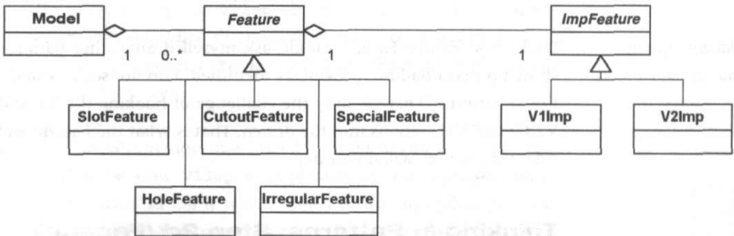
Figure 12-9 Applying the Bridge pattern to the problem.
