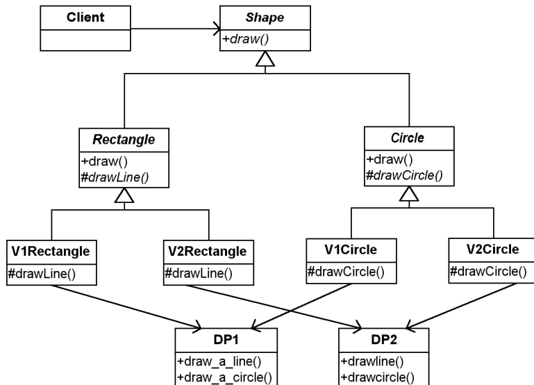
Figure 9-3 A straightforward approach: implementing two shapes and two drawing programs.
