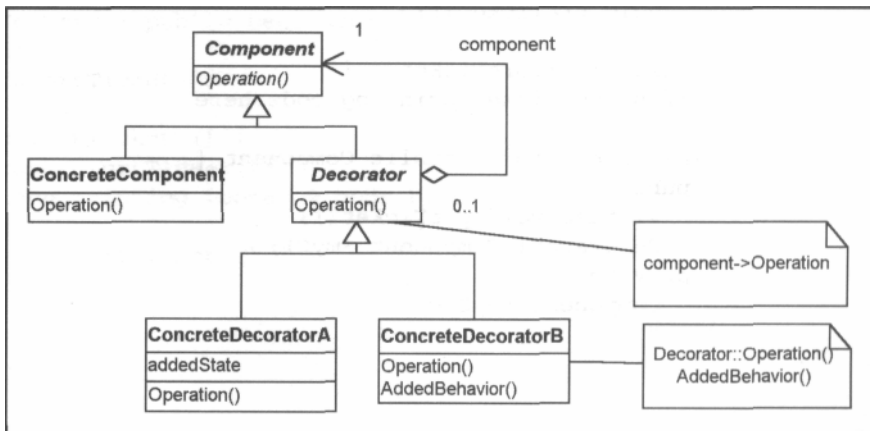
Figure 15-7 Standard, simplified view of the Decorator pattern.
