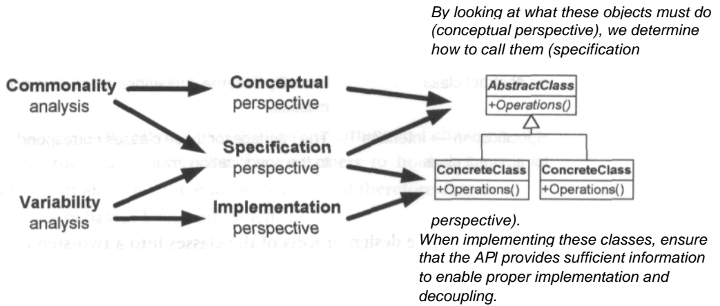
Figure 8-4 The relationship between commonality/variability analysis, perspectives, and abstract classes.
