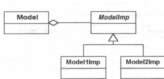
Figure 12-7 Using the Bridge pattern to handle the two model types.
