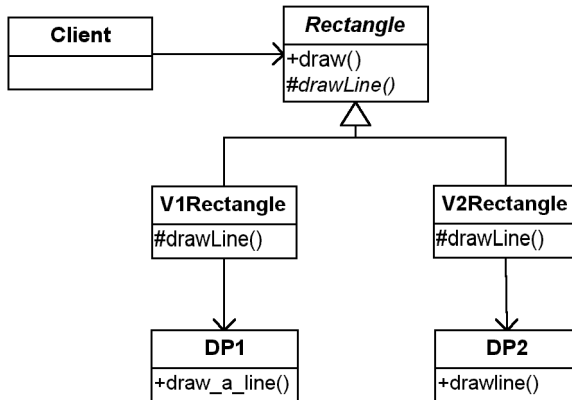
Figure 9-2 Design for rectangles and drawing programs (DP1 and DP2).
