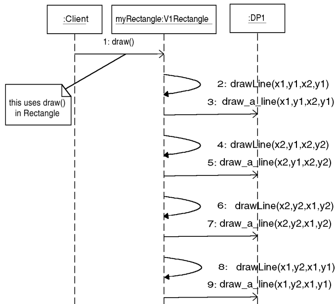
Figure 9-4 Sequence Diagram when have a V1Rectangle .
