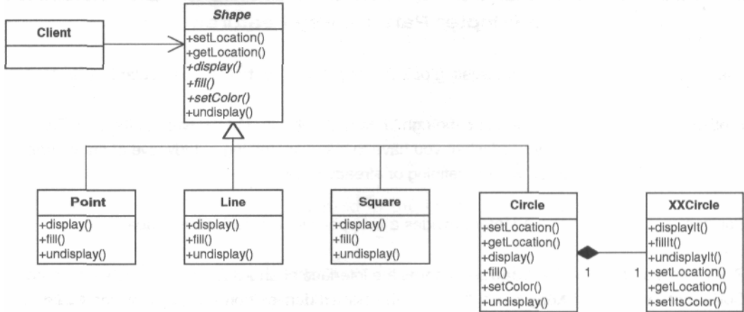
Figure 7-5 The Adapter pattern: Circle "wraps" XXCircle.
