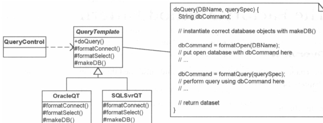
Figure 19-1 The Template Method ( doQuery ) using the Factory Method pattern ( makeDB ).
