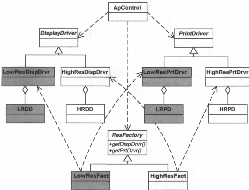
Figure 10-7 Solving the problem with the Abstract Factory and Adapter.
