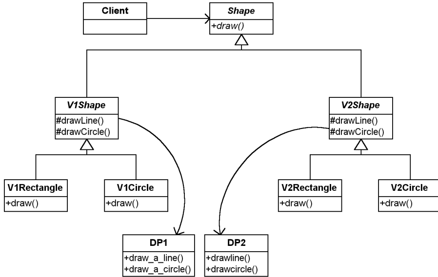
Figure 9-7 An alternative implementation.
