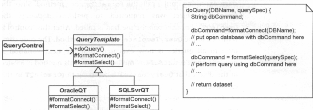
Figure 18-1 Using the Template Method pattern to perform a query.
