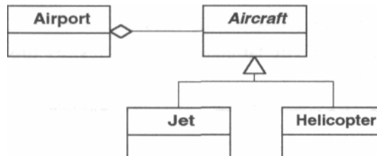
Figure 2-3 The Class Diagram showing the has-a relationship.
