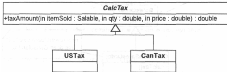
Figure 14-3 Encapsulating tax rules.
