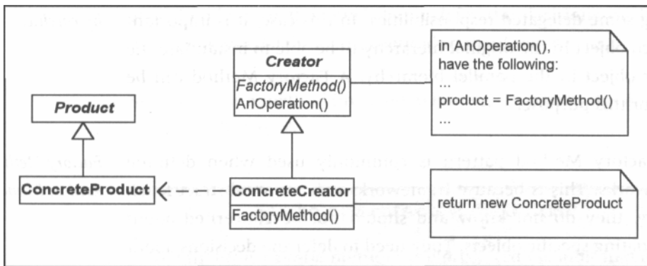
Figure 19-2 Standard, simplified view of the Factory Method pattern.
