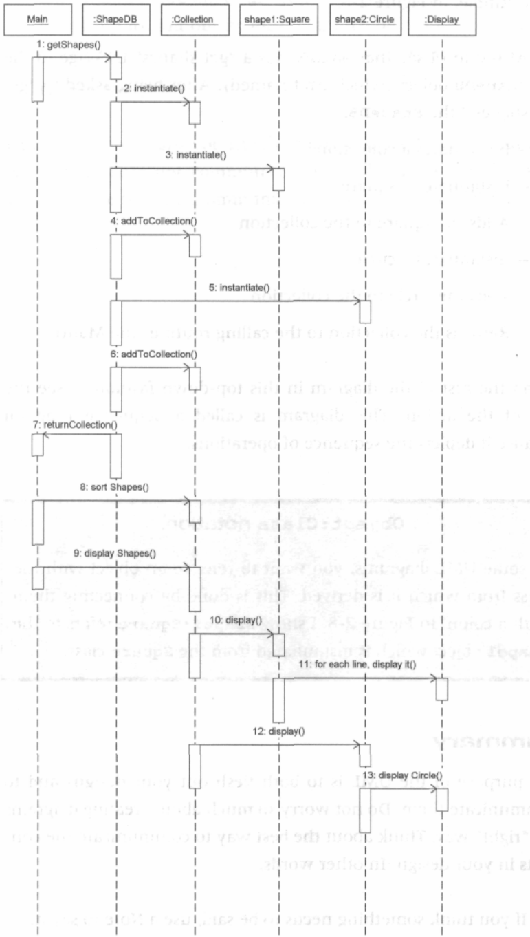
Figure 2-8 Sequence Diagram for the shapes program.
