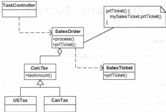
Figure 15-1 SalesOrder using SalesTicket.
