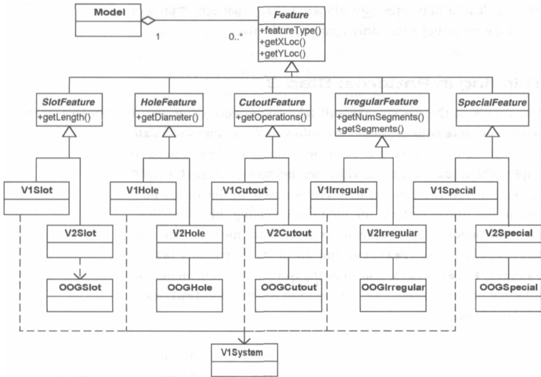
Figure 12-12 This was the first solution.
