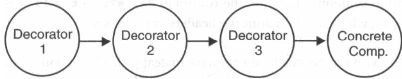
Figure 15-3 The Decorator chain.
