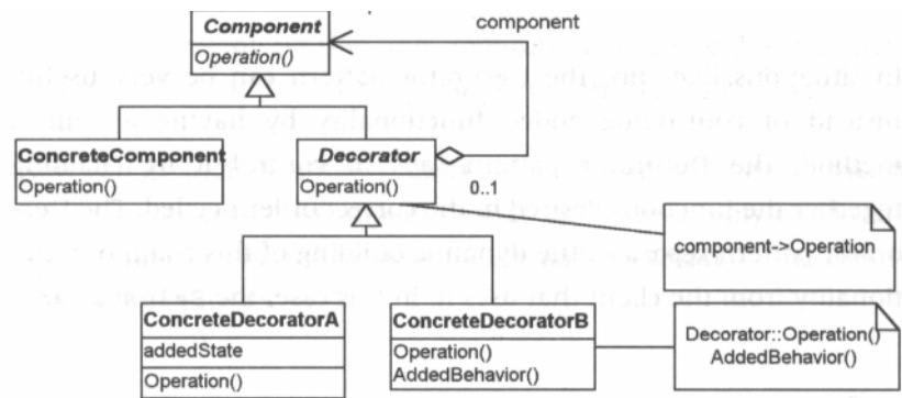
Figure 15-4 The Decorator pattern class diagram.
