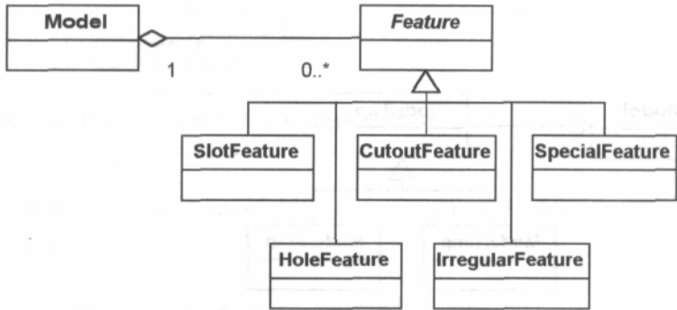
Figure 12-5 The Model design.
