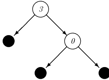
Figure 5.2: A binary tree of type tree .
