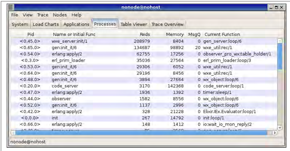
Figure 9-1. The Process Manager at startup
