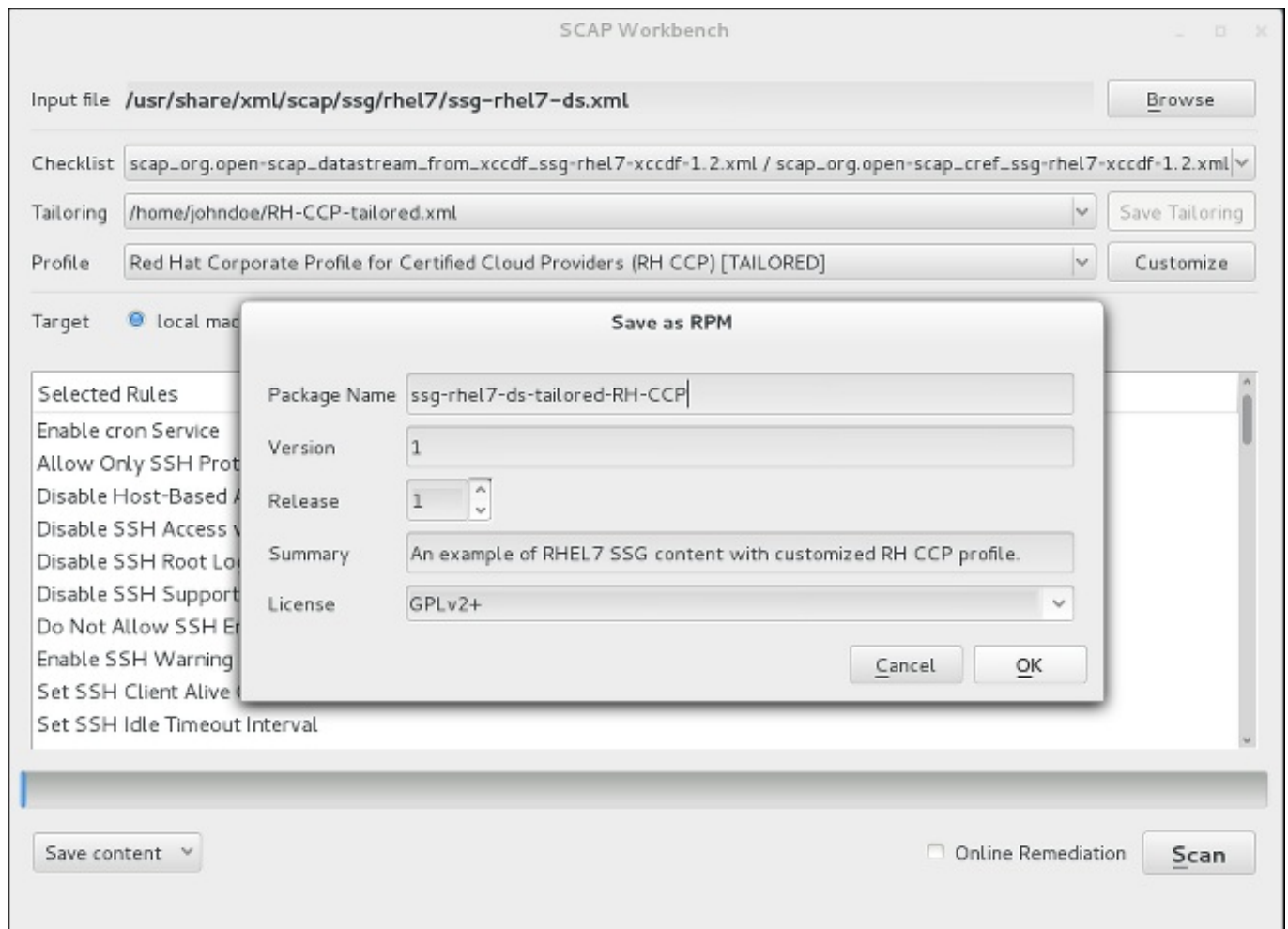
Figure 6.4. Saving the Current SCAP Content as an RPM Package
