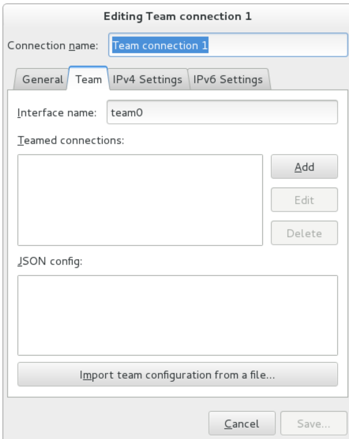
Figure 5.6. The NetworkManager Graphical User Interface Add a menu
