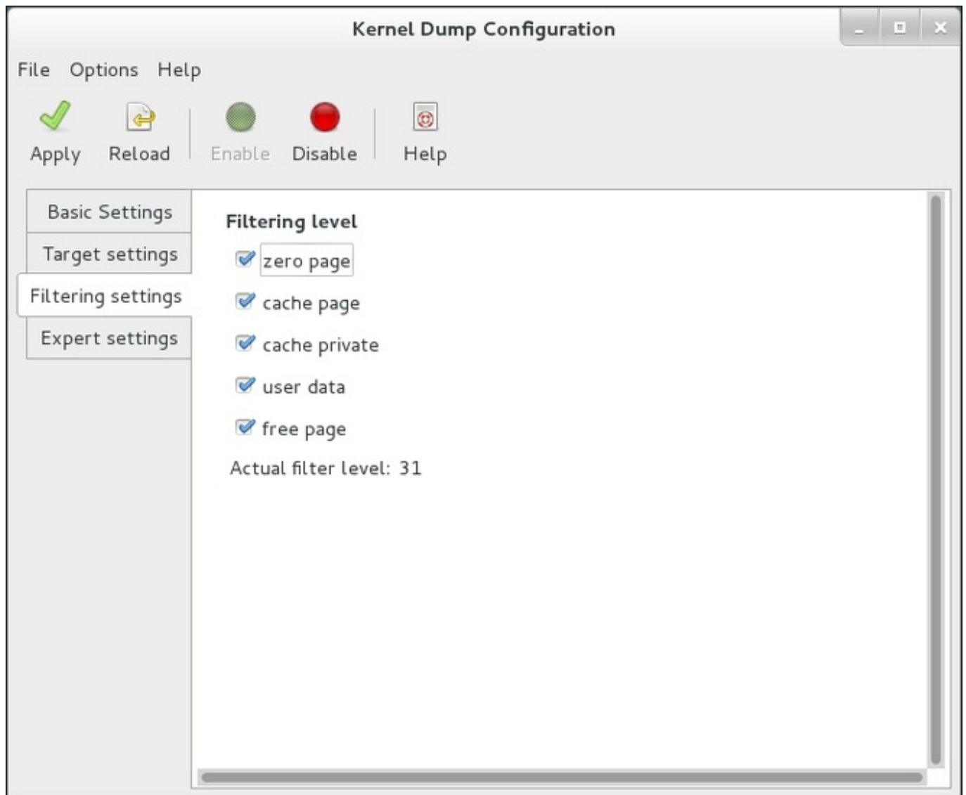
Figure 2.3. Filtering Settings
