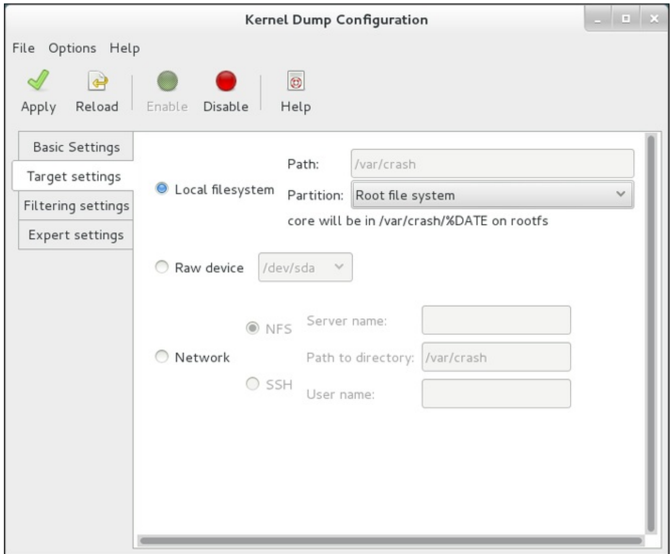
Figure 2.2. Target Settings
