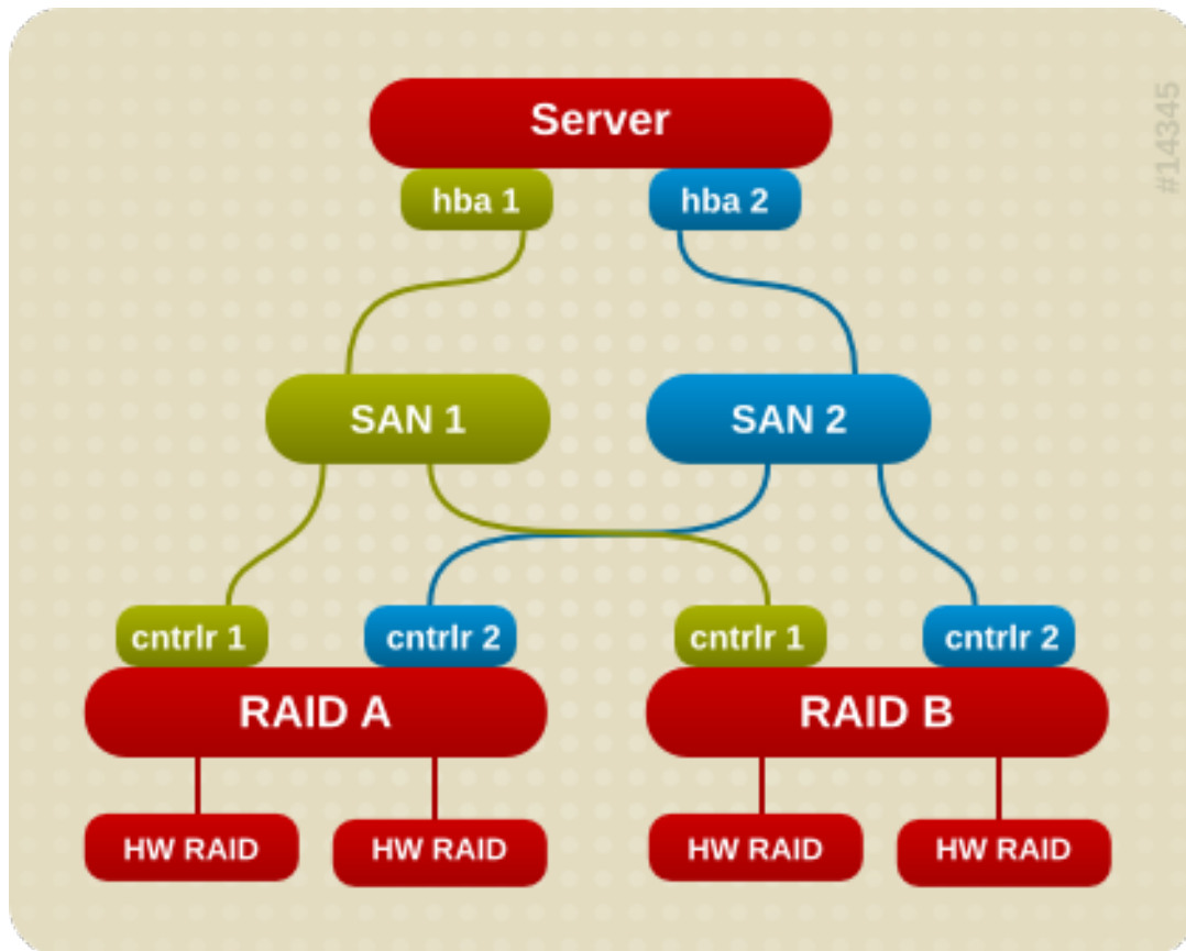
Figure 1.2. Active/Passive Multipath Configuration with Two RAID Devices
