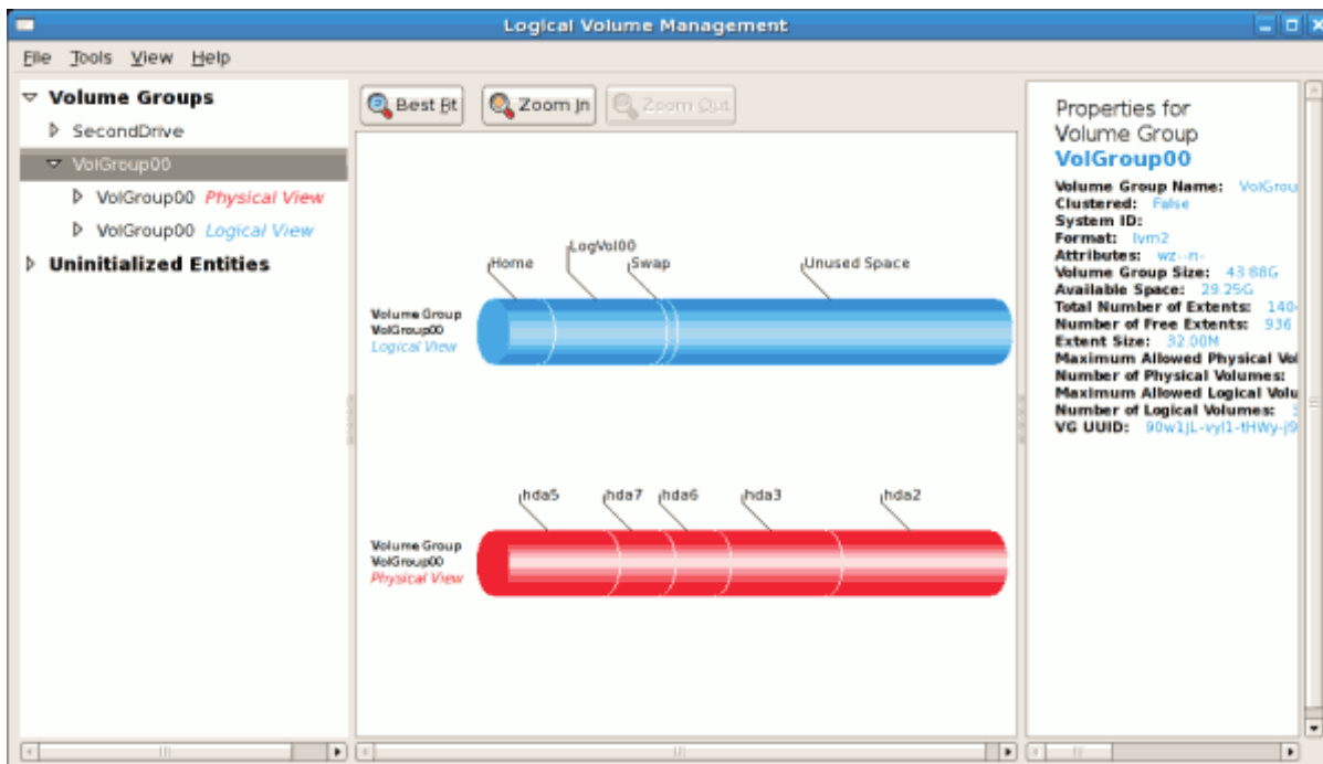
Figure 14.9. Logical view of volume group
