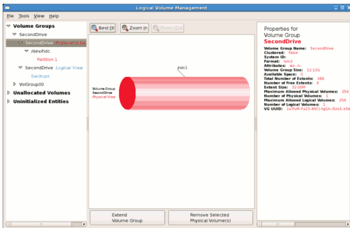
Figure 14.14. Physical view of new volume group
