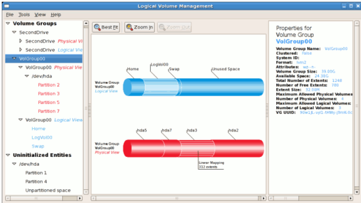
Figure 14.12. Logical and physical view of volume group
