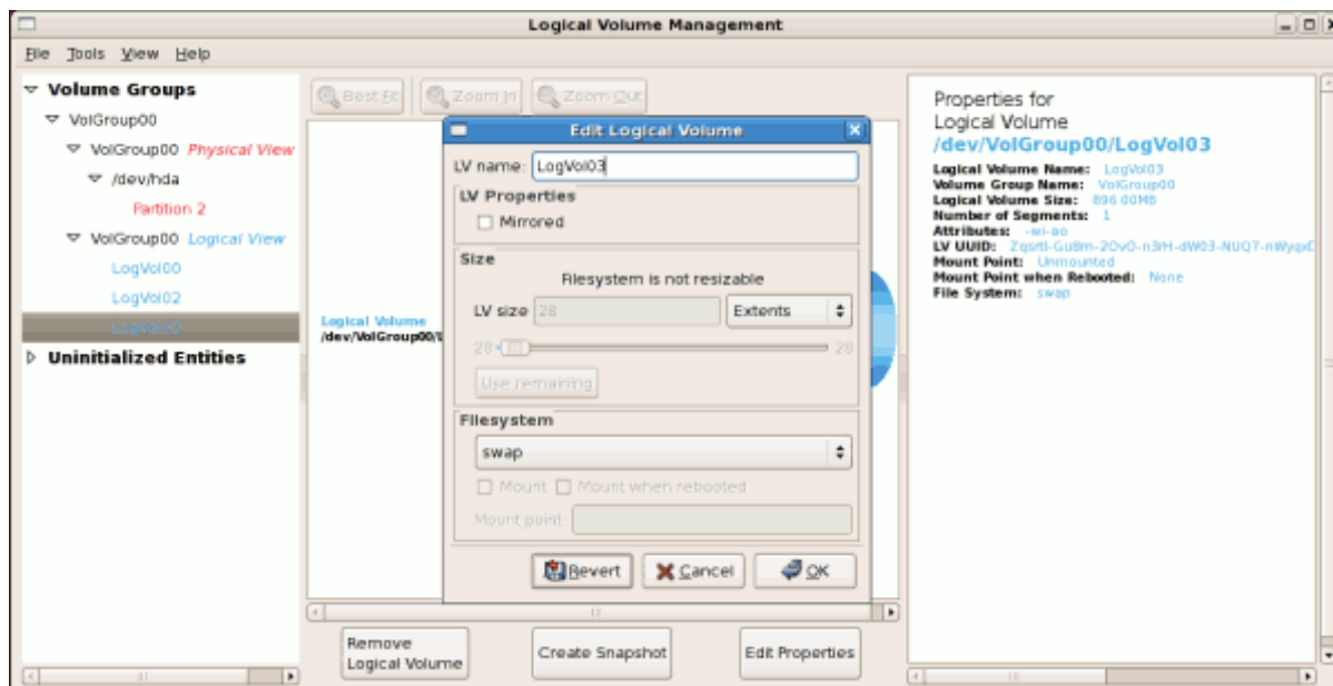
Figure 14.6. Edit Logical Volume
