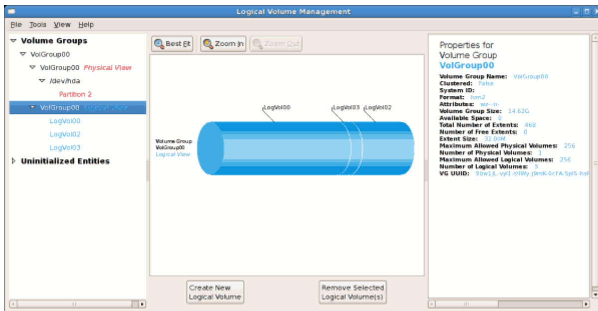
Figure 14.5. Logical View Window
