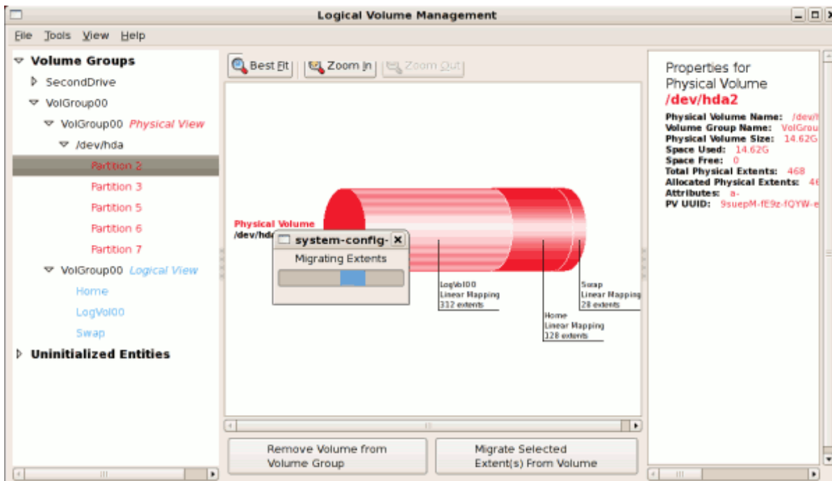
Figure 14.11. Migrating extents in progress
