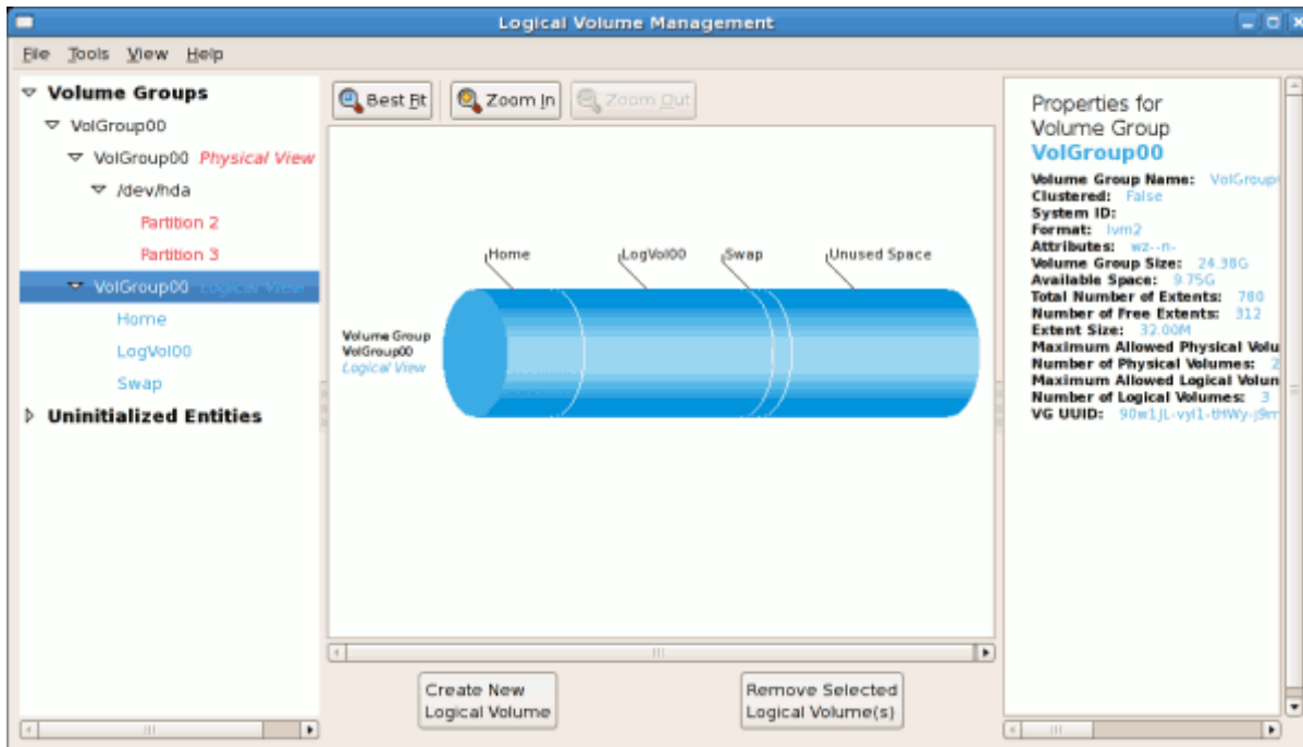
Figure 14.8. Logical view of volume group
