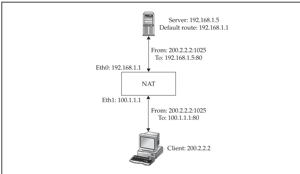
Figure 13-2. Using DNAT on a connection
