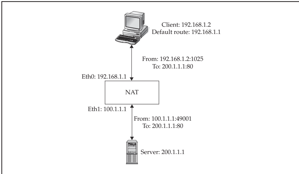
Figure 13-1. Using SNAT on a connection
