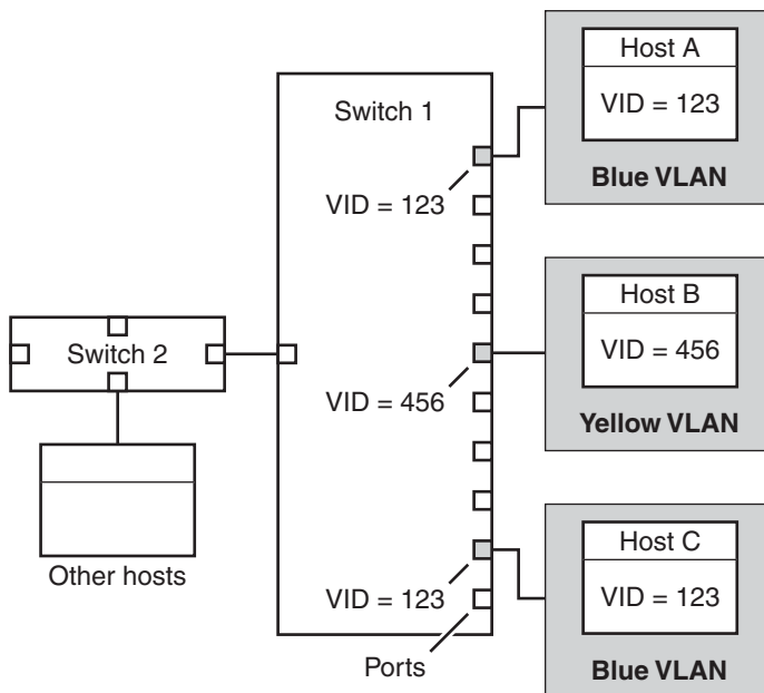
FIGURE 6–2 Switch Configuration for a Network with VLANs
