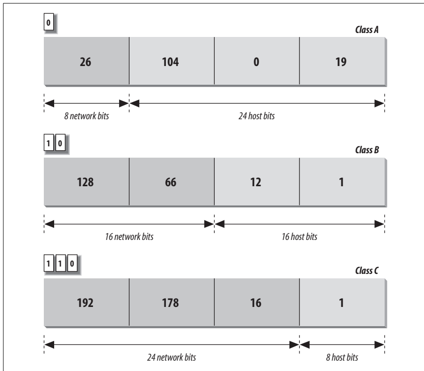
Figure 2-2. IP address structure
