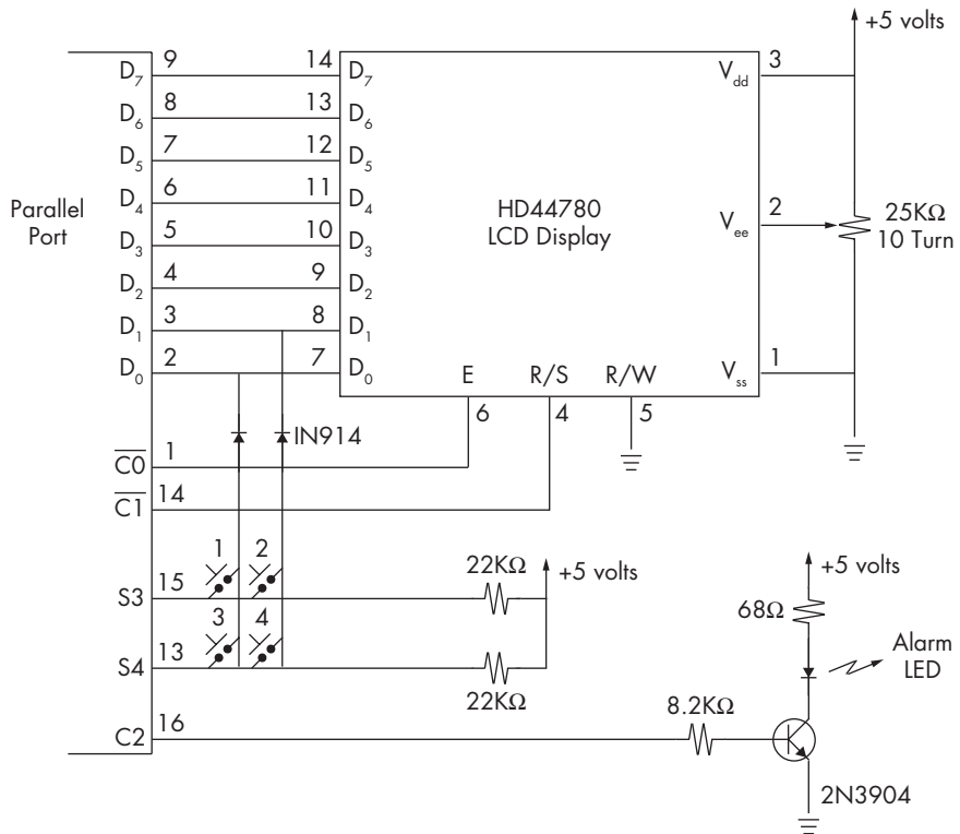
Figure 10-7: Schematic of the Laddie front panel
