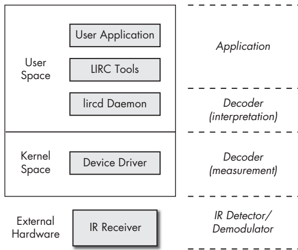
Figure 12-12: The LIRC architecture
