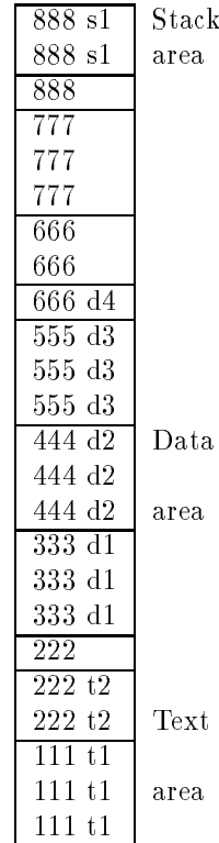
Virtual Address Space
