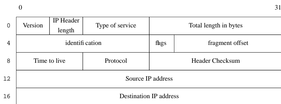
Figure 16-2: IP Header
