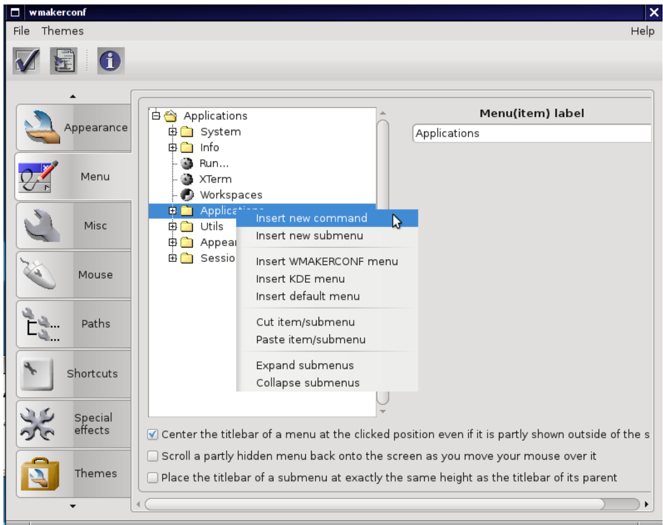
Figure 6.14b: Editing the Application Menu Using wmakerconf
