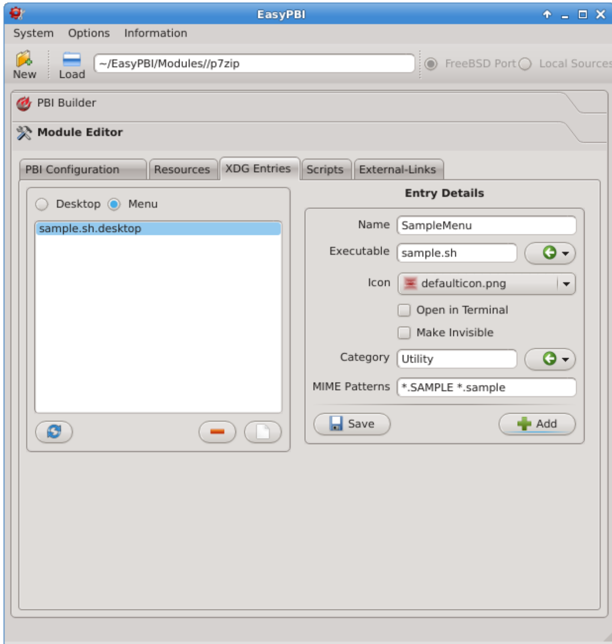
Figure 8.11: Menu Entry Details
