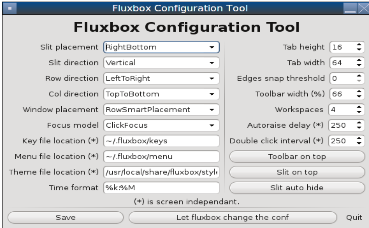
Figure 6.6c: Configuring Window Placement with fluxconf
