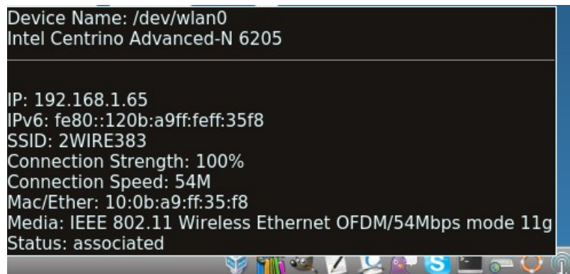
Figure 8.16a: Wireless Information in System Tray
