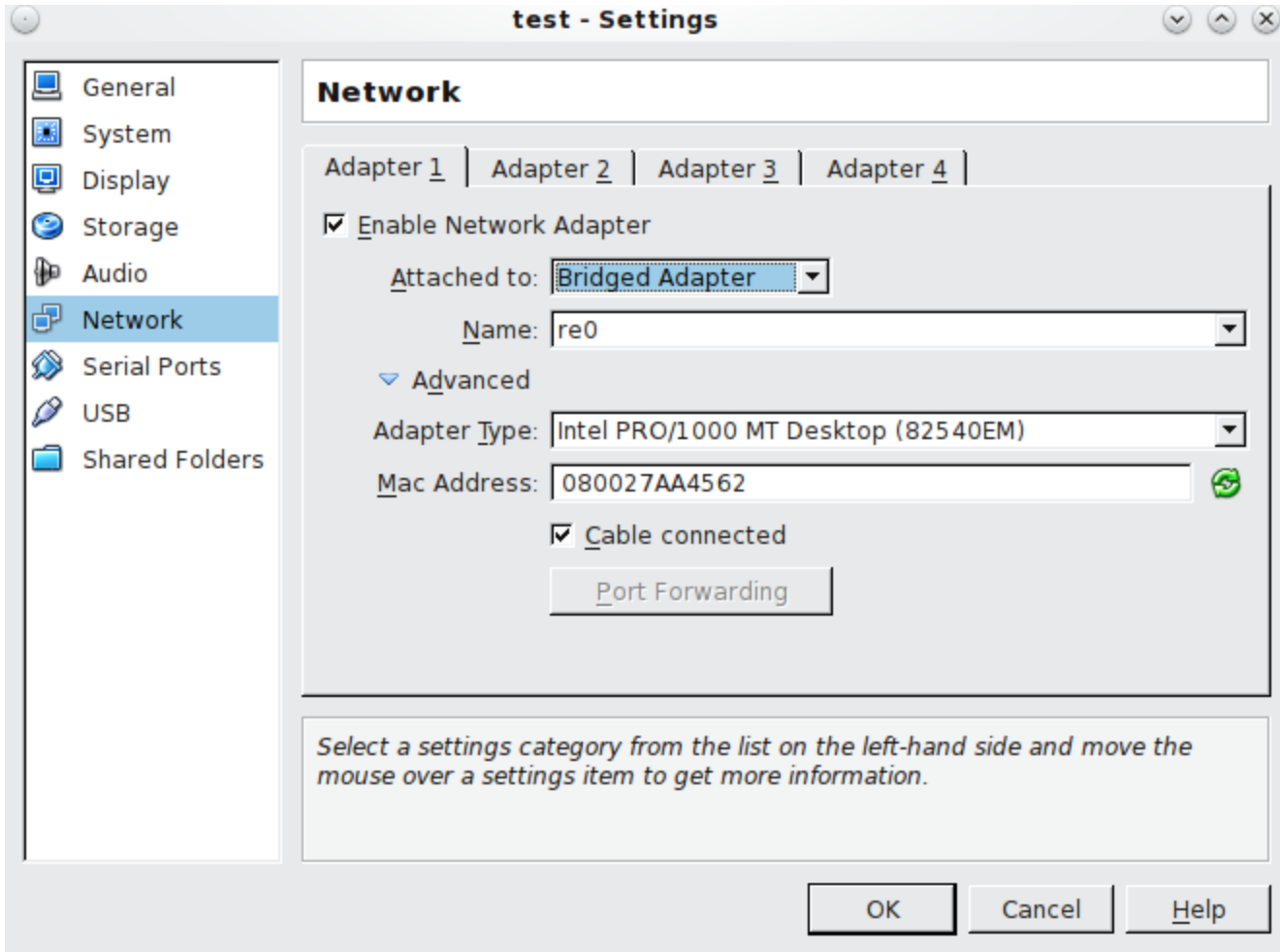
Figure 2.7i: Configuring a Bridged Adapter in VirtualBox
