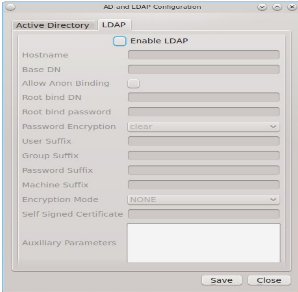
Figure 8.3b: Managing LDAP Client Settings
