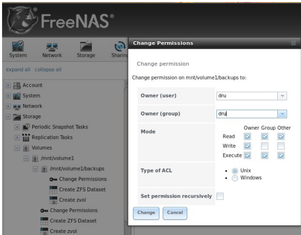
Figure 8.19m: Setting Permissions in FreeNAS® 9.1.1
