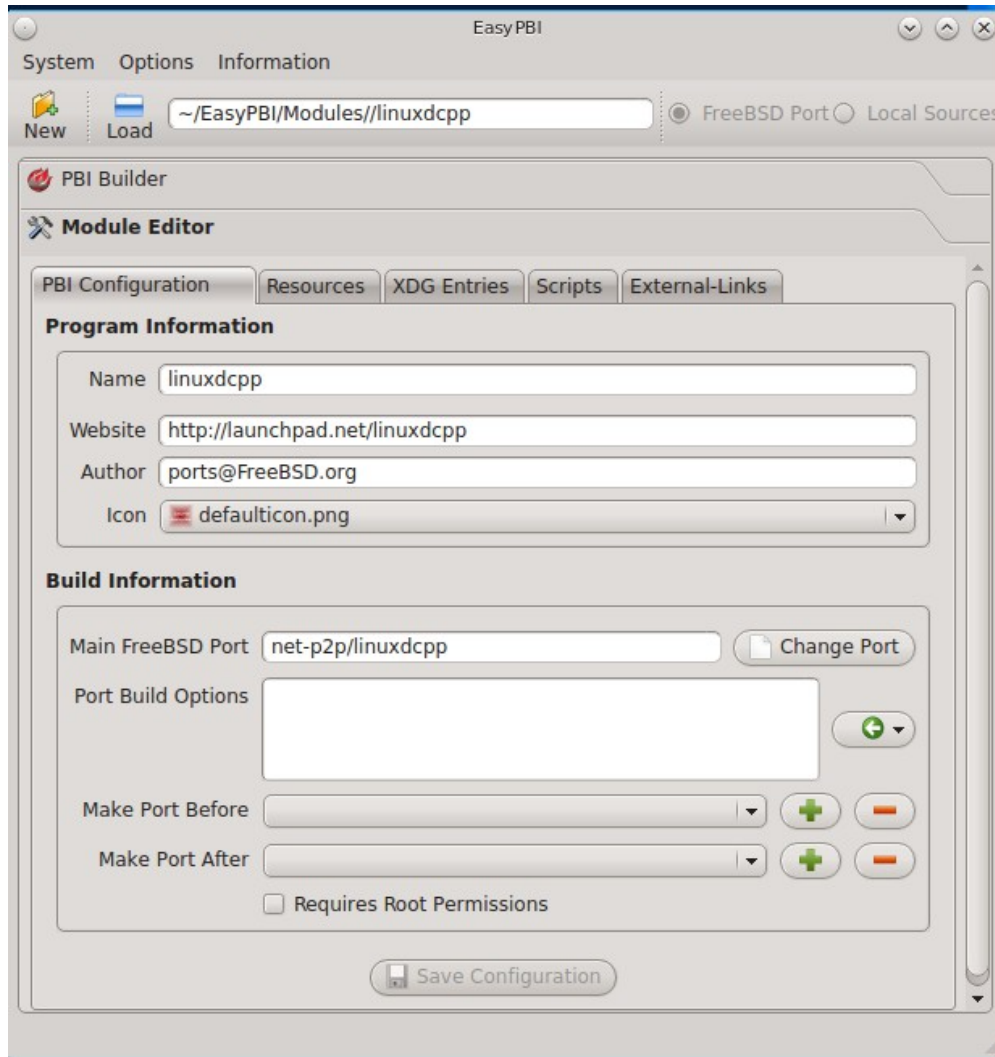
Figure 8.1d: Module Program Information
