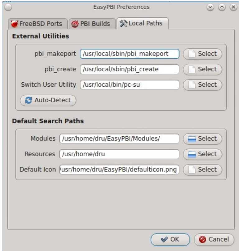
Figure 8.1g: Local Paths Settings
