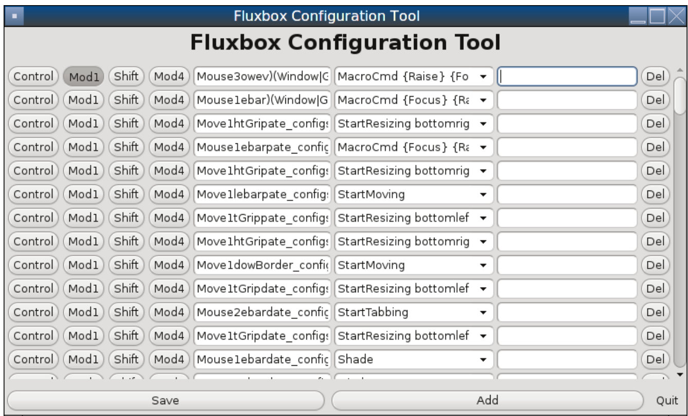
Figure 6.6d: Managing Keyboard Shortcuts with fluxkeys
