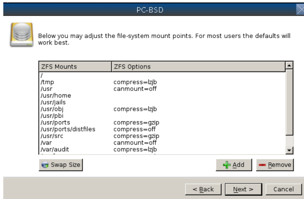
Figure 3.4f: Default ZFS Layout
