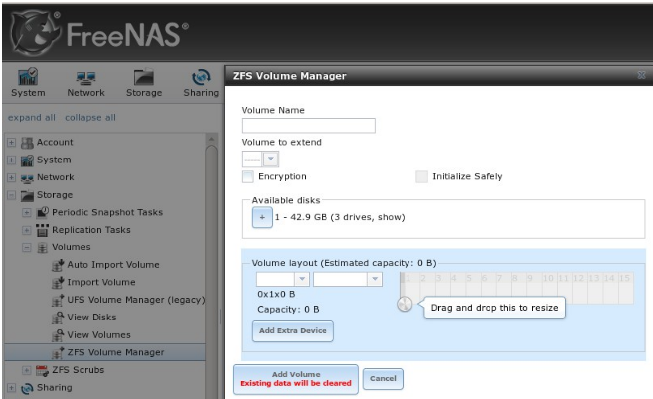
Figure 8.19j: Creating a ZFS Volume in FreeNAS® 9.1.1
