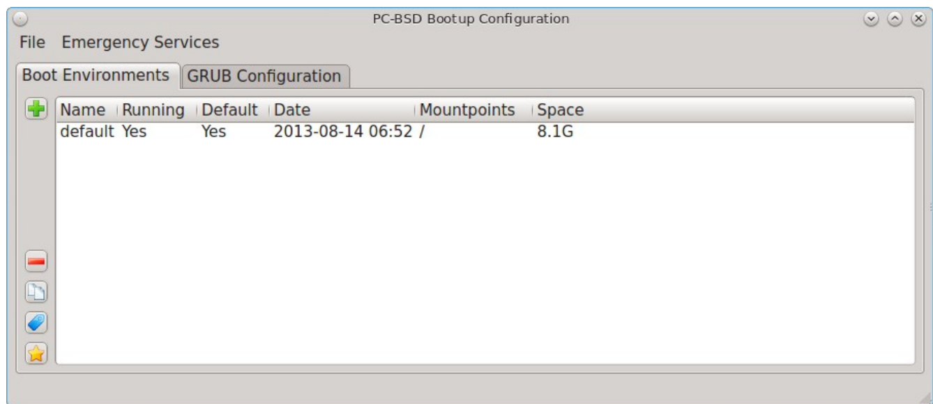
Figure 8.4a: Managing Boot Environments
