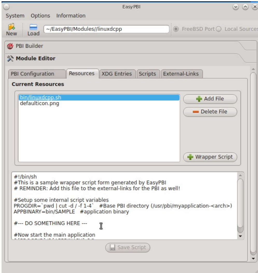
Figure 8.1j: Edit the Automatically Generated Script
