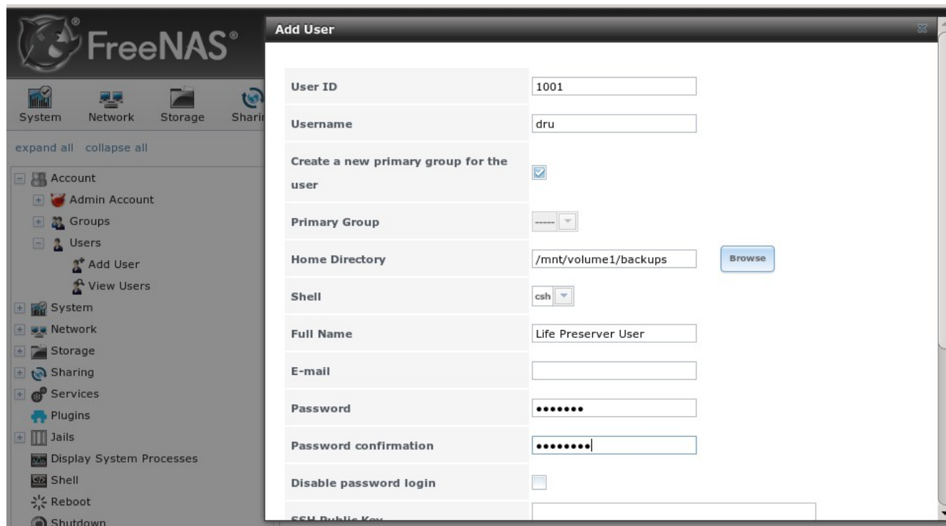
Figure 8.19l: Creating a User in FreeNAS® 9.1.1
