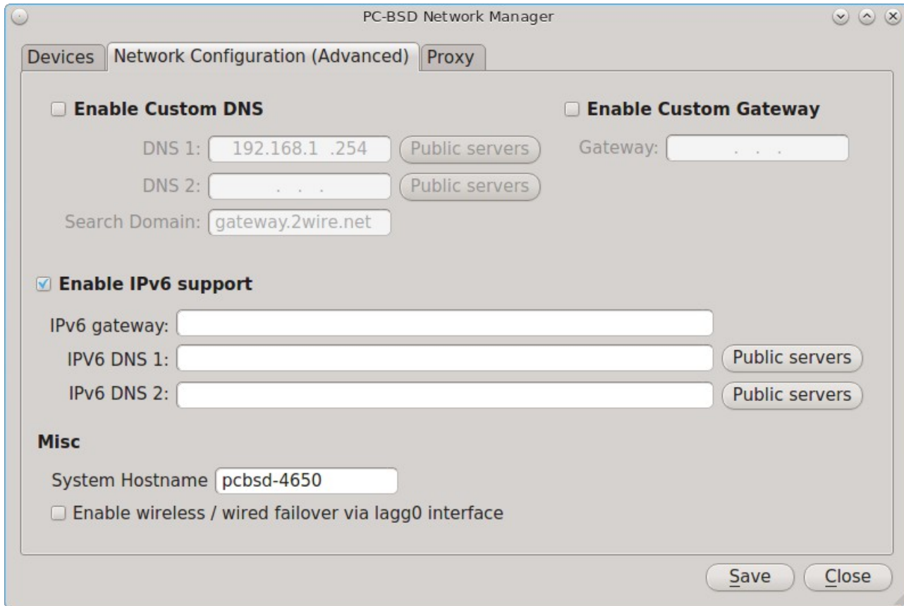
Figure 8.16m: Network Configuration (Advanced) tab of the Network Configuration Utility
