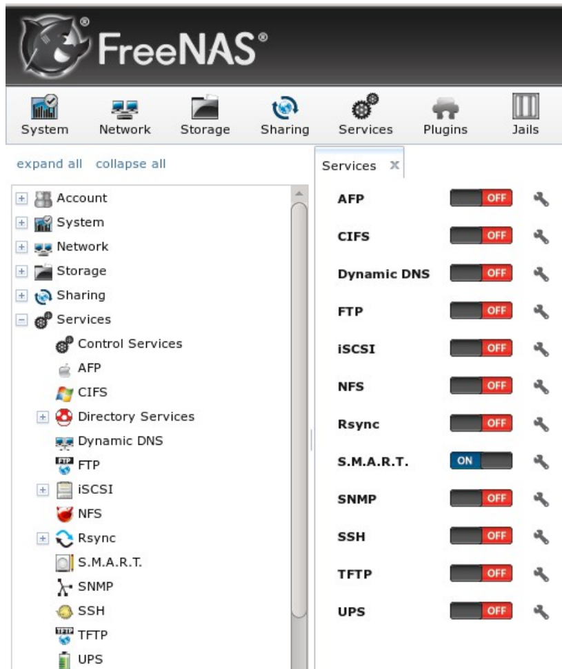
Figure 8.19n: Start SSH in FreeNAS® 9.1.1
