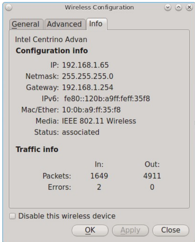
Figure 8.16l: Info Tab of a Wireless Interface
