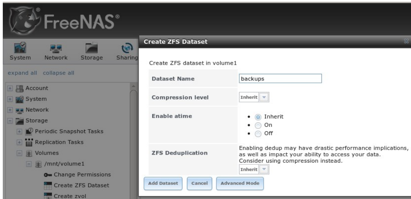
Figure 8.19k: Creating a ZFS Dataset in FreeNAS® 9.1.1
