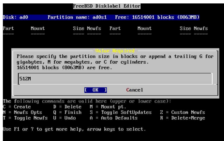
Figure 2-21. Edit Root Partition Size
