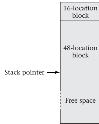
Figure A.1: A stack grows downward, occupying the highest addresses in the region used to store it. The stack pointer points at the “top” of the stack, that is, the most recently allocated block of space. In this example, blocks of size 16 and 48 were allocated, so the stack pointer points at the 64th location from the end of the memory region.
