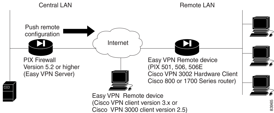
Figure 8-1 Using the PIX Firewall as an Easy VPN Server
