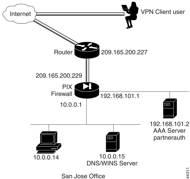
Figure 8-2 Cisco Easy VPN Remote Device Access
