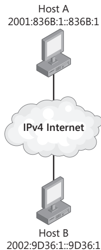
Figure 13-2 An example 6to4 configuration
