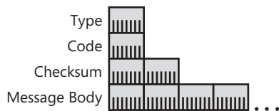
Figure 5-1 The structure of ICMPv6 messages
