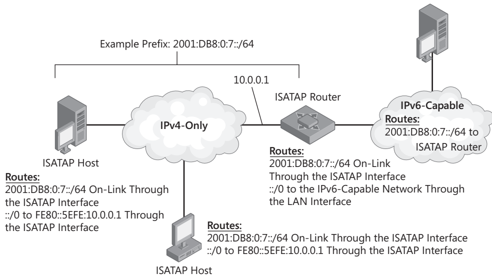
Figure 12-5 ISATAP routing example
