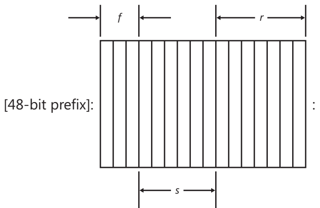
Figure 3-10 The subsetting of a subnet ID
