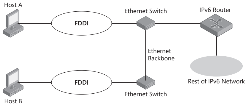
Figure 6-8 A mixed-media configuration
