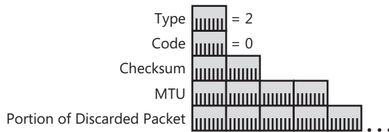
Figure 5-3 The structure of the Packet Too Big message
