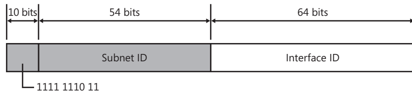
Figure 3-4 The structure of the site-local address
