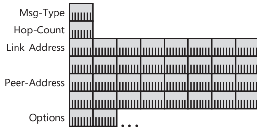
Figure 8-6 DHCPv6 messages between relay agent and server
