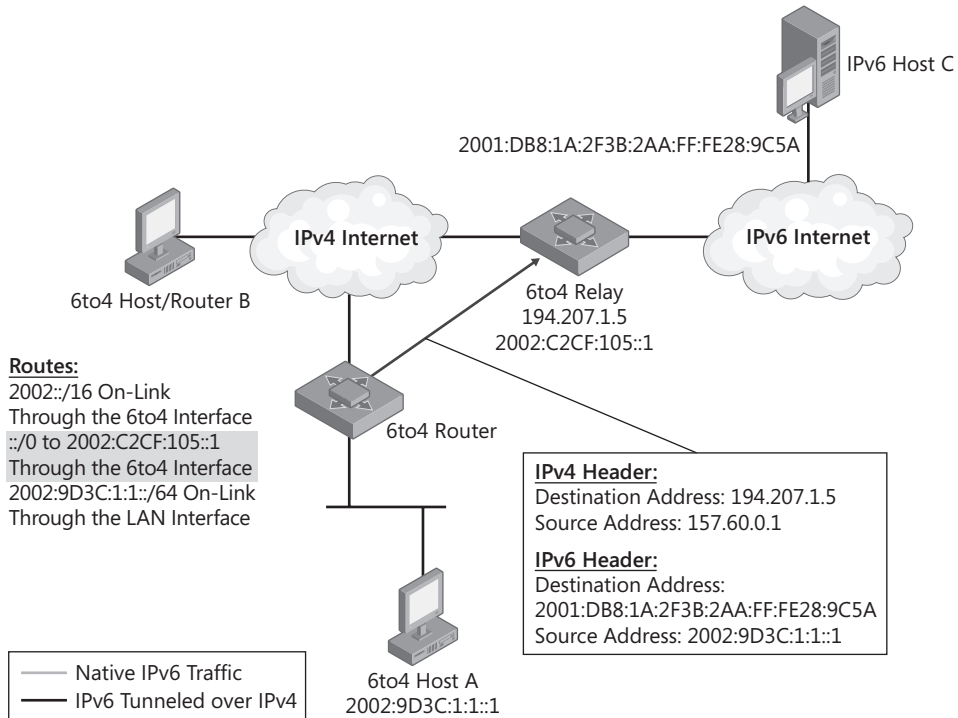
Figure 13-10 6to4 host to IPv6 host communication—Part 2
