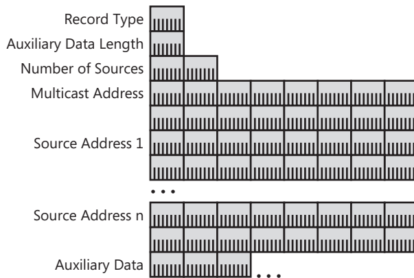
Figure 7-7 The structure of the multicast address record
