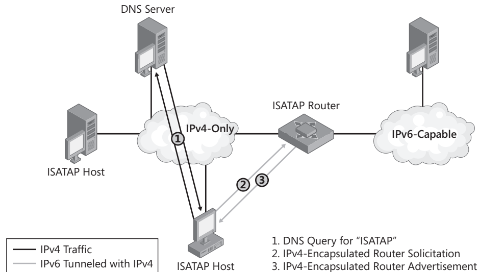
Figure 12-3 Performing router discovery with an ISATAP router
