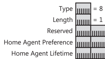
Figure F-12 The structure of the Home Agent Information option
