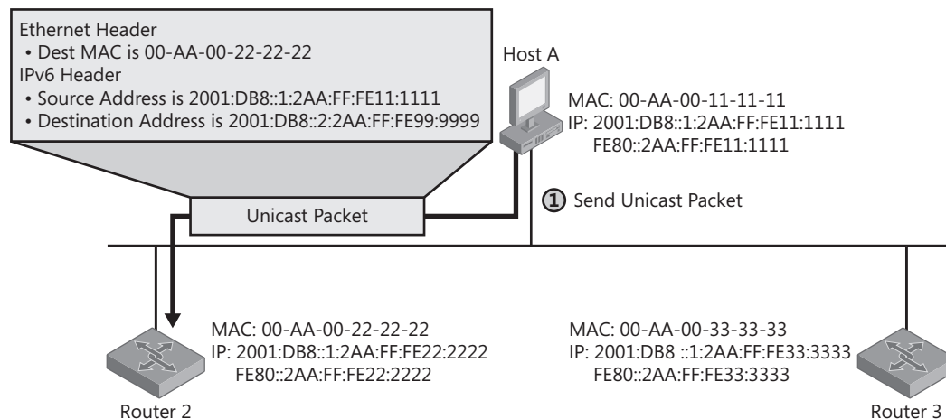
Figure 6-25 The unicast packet sent to the router
