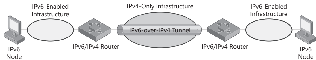
Figure 11-6 Router-to-router tunneling
