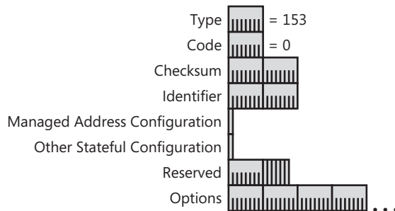
Figure F-8 The structure of the ICMPv6 Mobile Prefix Advertisement message
