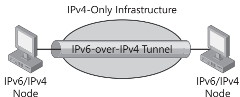
Figure 11-8 Host-to-host tunneling
