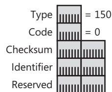
Figure F-5 The structure of ICMPv6 Home Agent Address Discovery Request message
