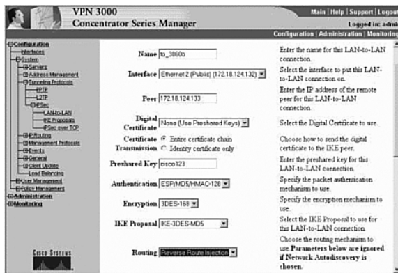
Figure 9-4 Configuration / System / Tunneling Protocols / IPSec / LAN-to-LAN / Modify
