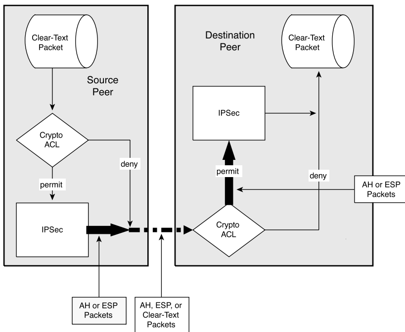
Figure 2-12 Crypto ACLs
