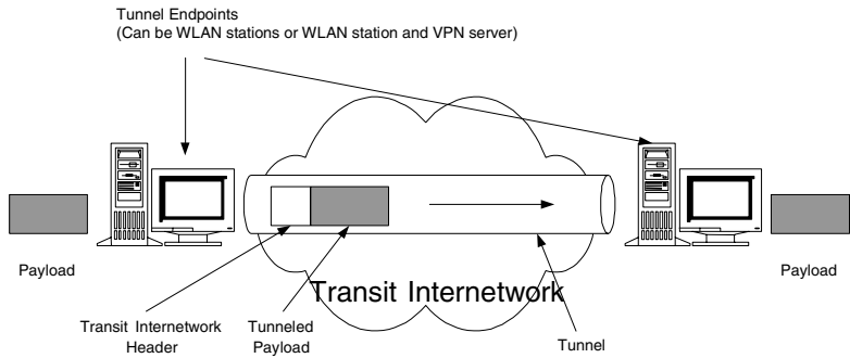
Figure 4.2 Tunneling.
