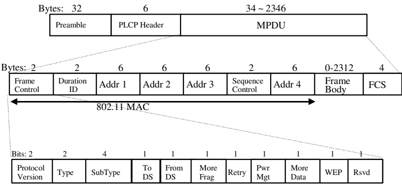
Figure 3.6 MAC frame format [1, 4].
