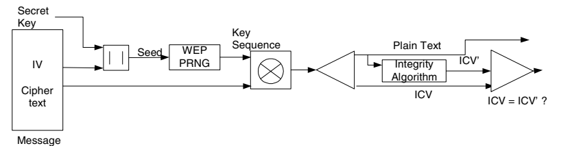
Figure 3.19 WEP decipherment block diagram [1] (reprinted with permission from IEEE 802.11-1999).
