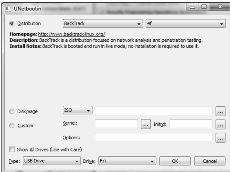
Figure 7-3 UNetbootin interface
