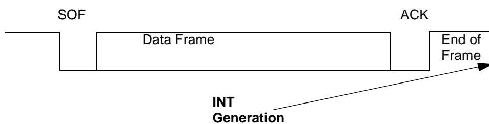
Figure 12. DATA frame
