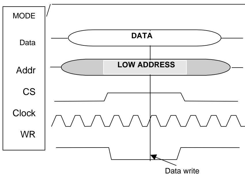
Figure 7. Mode 1 Write Cycle
