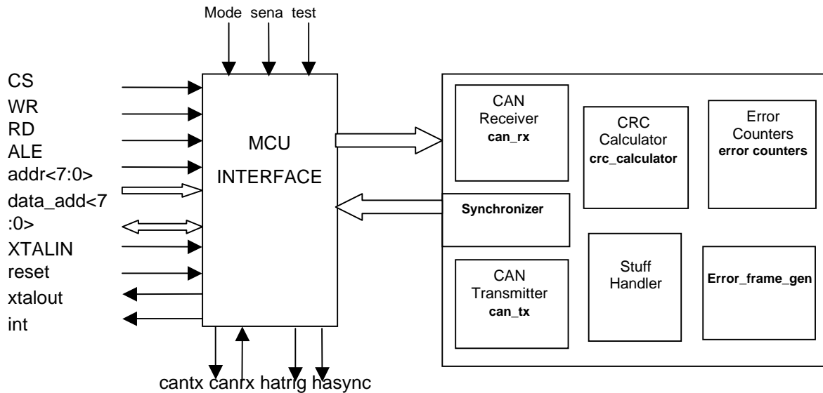
Figure 1. Block Schematic of AT7908E
