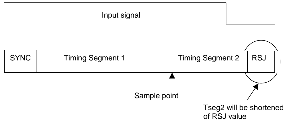
Figure 4. Shortening a Bit Period
