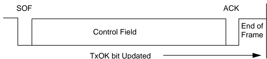
Figure 13. Remote frame
