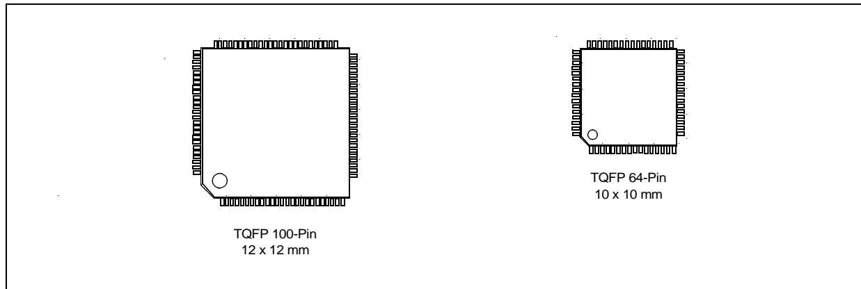
FIGURE 1: PIC32MX3XX/4XX PACKAGE OUTLINE DRAWING
