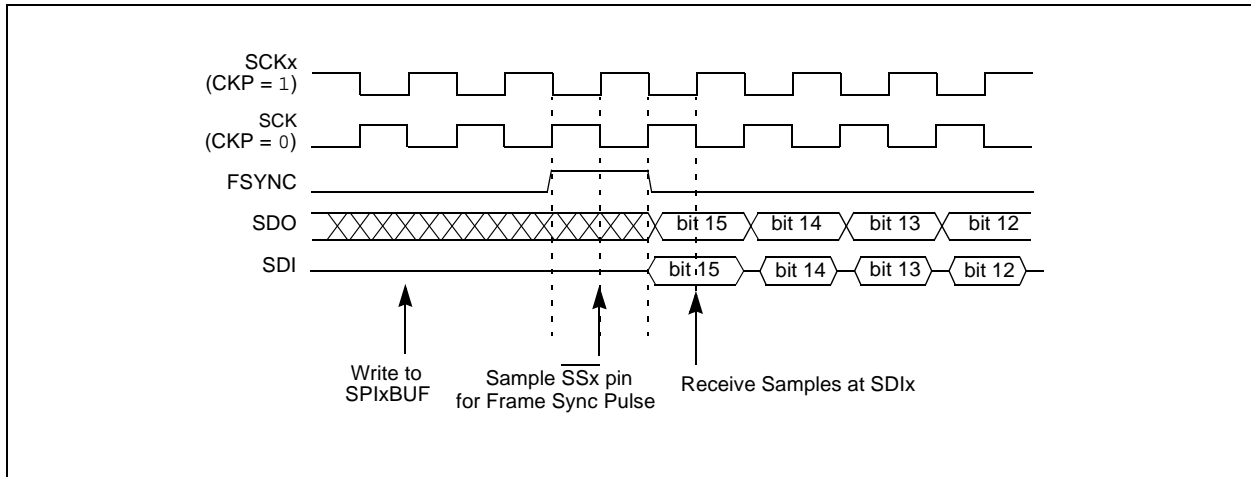
FIGURE 17-7: SPI MASTER, FRAME SLAVE MODE MODE32 = 0 , MODE16 = 1 , SPIFE = 0 , FRMPOL = 1
