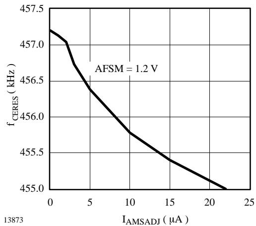
Figure 14. Pulling characteristic
