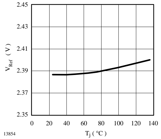
Figure 42. Temperature characteristic of V_{Ref}
