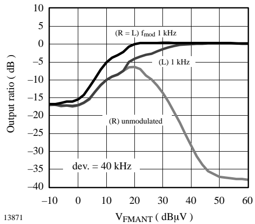
Figure 49. Channel-separation characteristic
