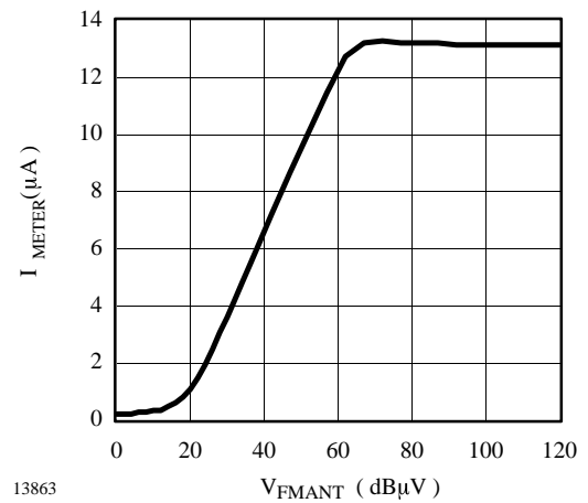
Figure 54. FM field-strength characteristic
