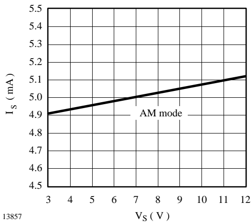
Figure 41. Supply-current characteristic
