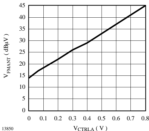
Figure 29. Adjustable FM stop-signal sensitivity
