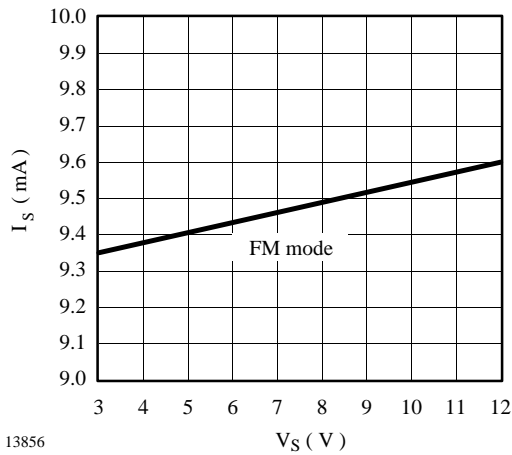
Figure 40. Supply-current characteristic
