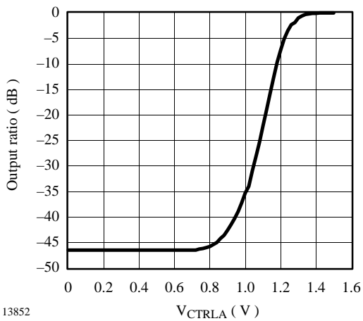
Figure 31. Mute function
