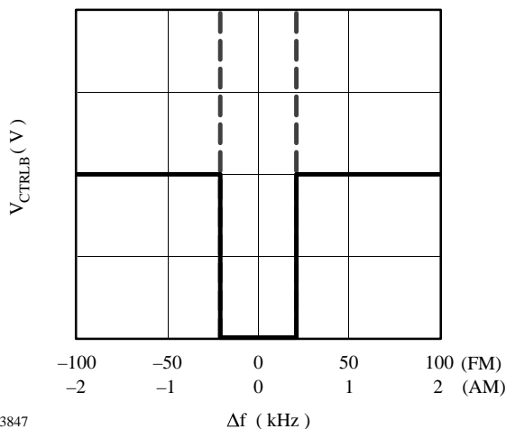
Figure 38. Stop signal
