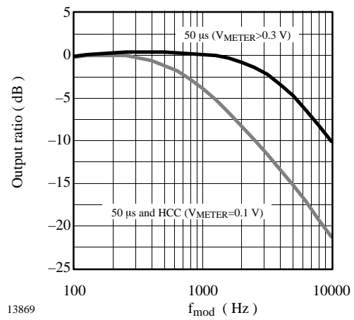
Figure 44. High-cut control (HCC)
