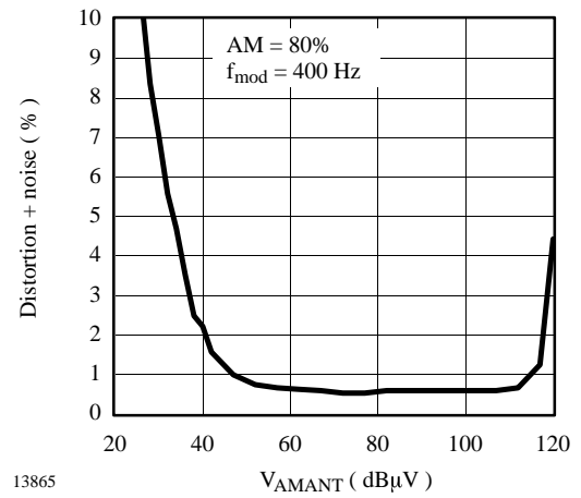
Figure 55. AM distortion and noise characteristic
