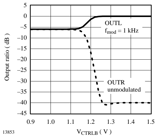
Figure 33. Forced mono function
