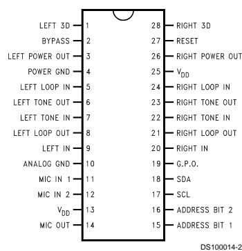
Top View Order Number LM4832N, LM4832M See NS Package Number N28B for DIP See NS Package Number M28B for SOIC
