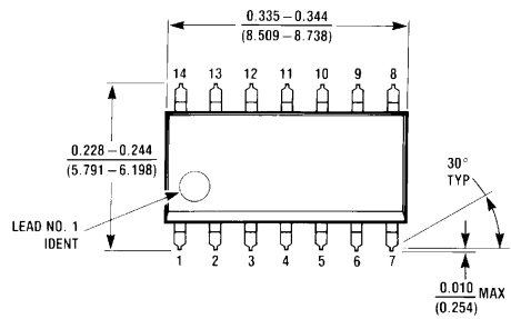
Ceramic Dual-In-Line Package (J) Order Number LM359J NS Package Number J14A
