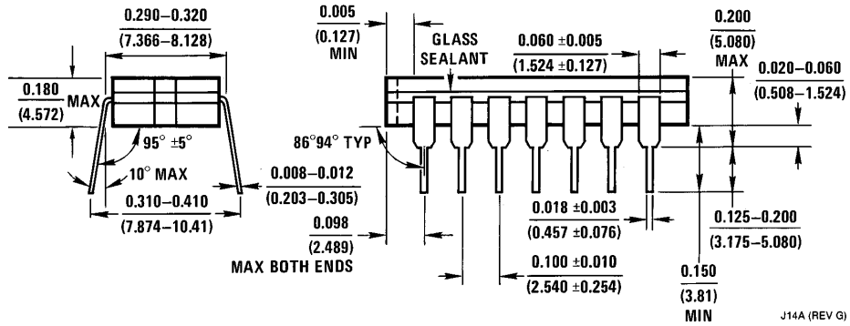
Ceramic Dual-In-Line Package (J) Order Number LM359J NS Package Number J14A
