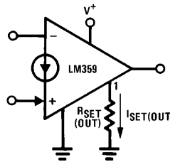
FIGURE 6. Establishing the Output Set Current
