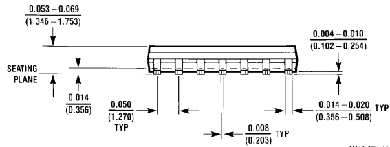
S.O. Package (M) Order Number LM359M NS Package Number M14A
