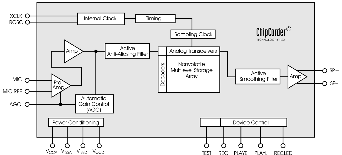
Figure i: ISD1520 Block Diagram
