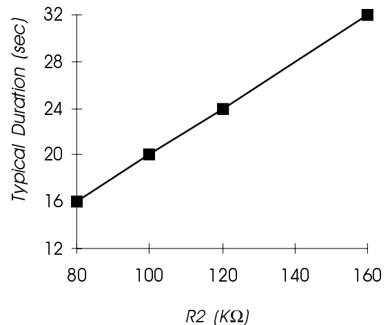
Chart 1: ISD1520 Duration versus R2 ( R_{\text{OSC}} ) at T_{\text{A}} = 25^{\circ}\text{C} and 5.0 V
