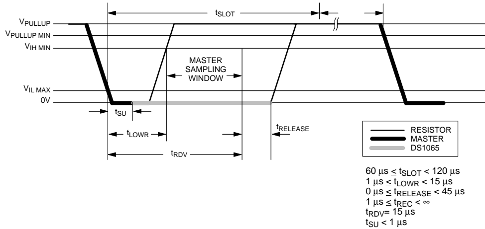
READ DATA TIME SLOT Figure 16
