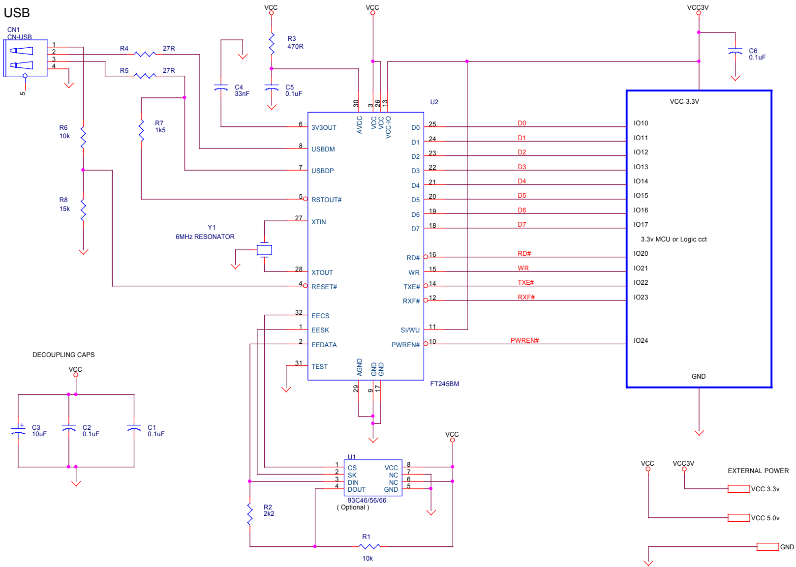
FT245BM 3.3v SELF POWERED EXAMPLE
