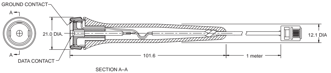
a) Hand Grip Probe, dimensions
