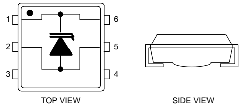
TSOC SURFACE MOUNT PACKAGE
