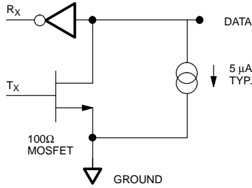
DS1986 EQUIVALENT CIRCUIT Figure 6
