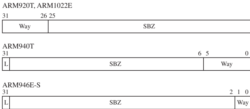
Figure 12.13 CP15:c9 register format used when locking data in cache by reference to its way.
